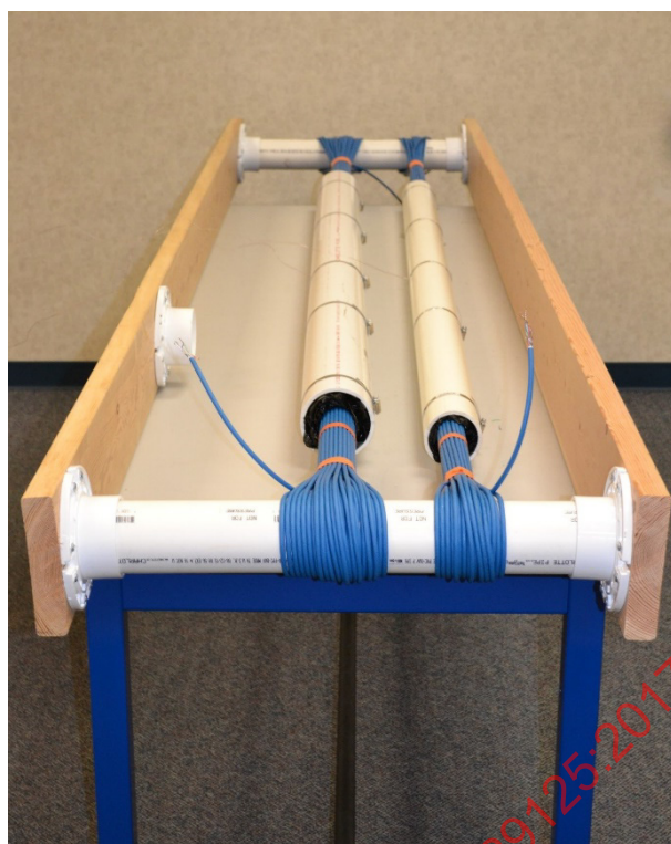
Figure F.4 – Test set-up for cable bundles in conduit
