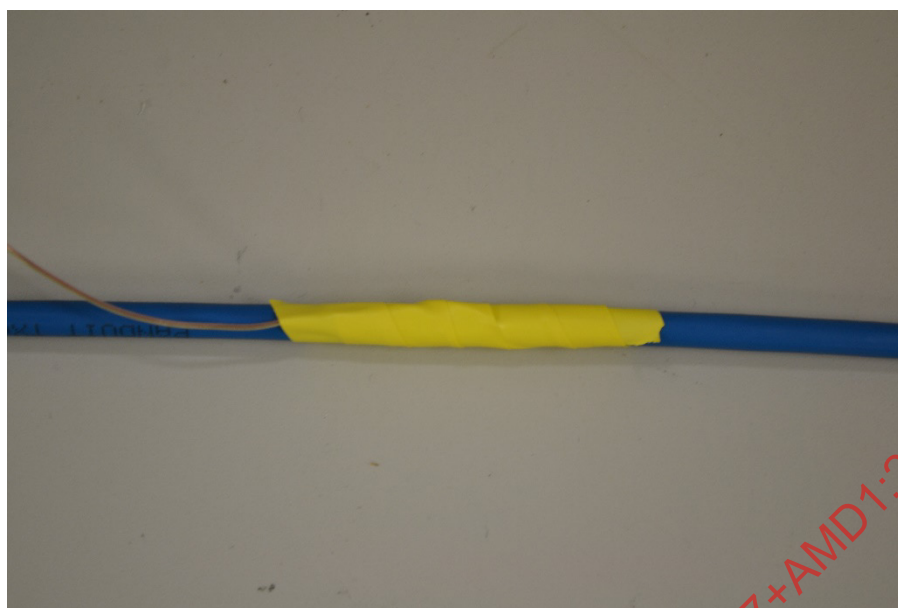
Figure F.2 – Securing of the thermocouple
