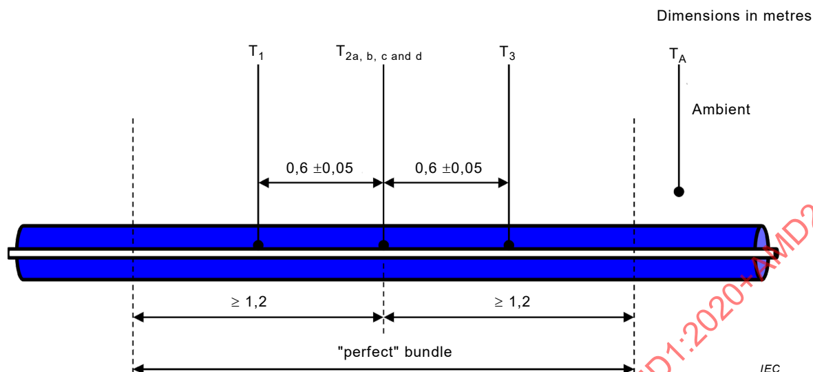
Figure E.2 – "Perfect bundle" and thermocouple configuration
