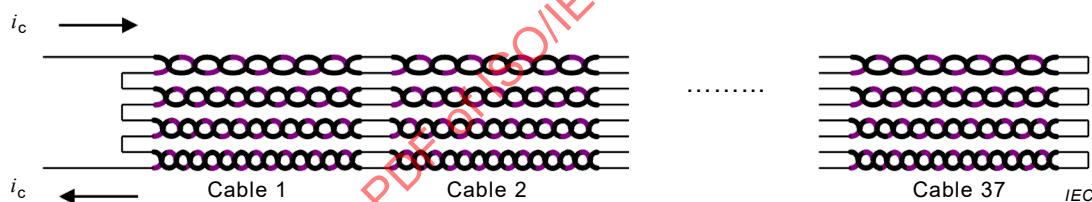
Figure E.3 – 4-pair cabling conductor configuration
