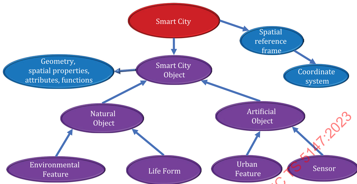
Figure 3 — Further decomposition of smart city objects
