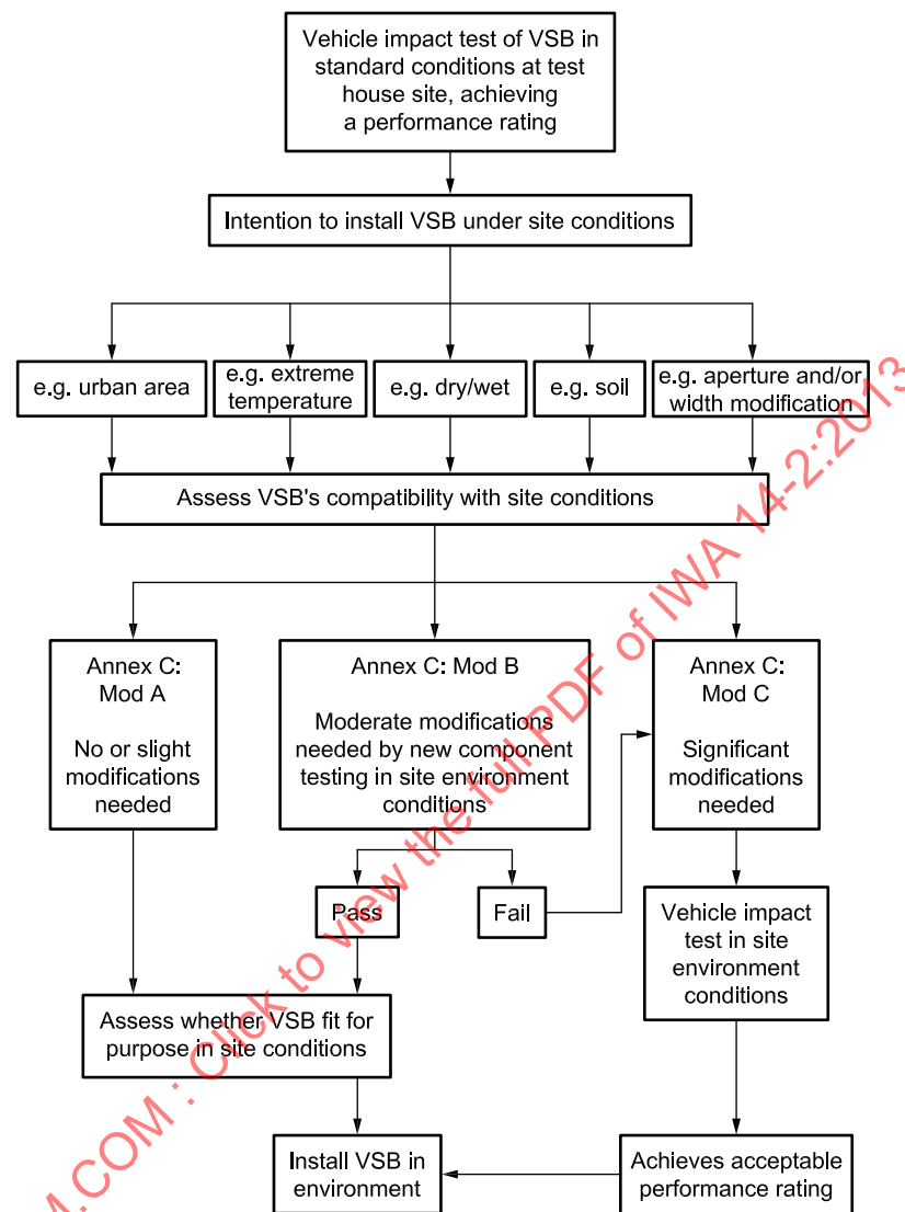
Figure 1 Process for assessing a VSB for use under site conditions (informative)
