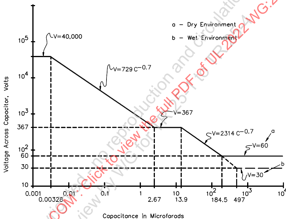
Figure 9.1 Limits for Voltage Across Capacitance
