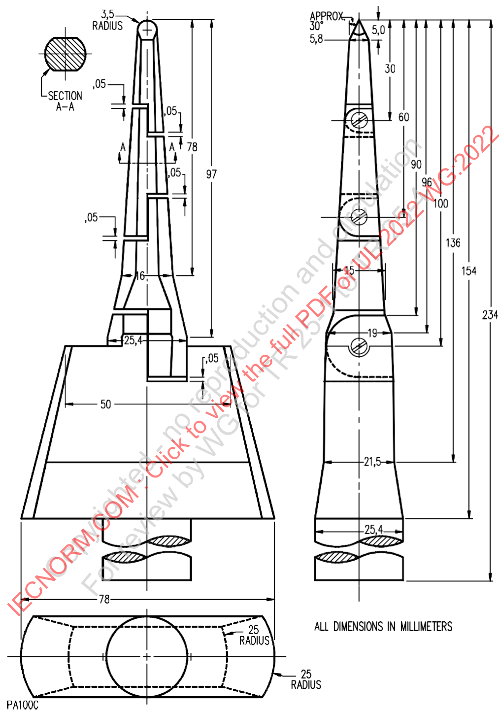
Figure 8.1 Articulated Probe
