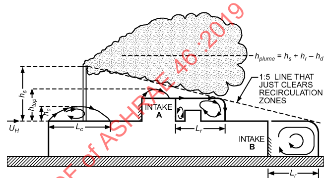
Fig. 1 Flow Recirculation Regions and Exhaust Parameters (Wilson 1982)
