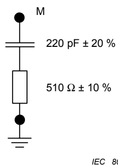
Figure 6 – Artificial hand, RC element (see 7.3.5)
