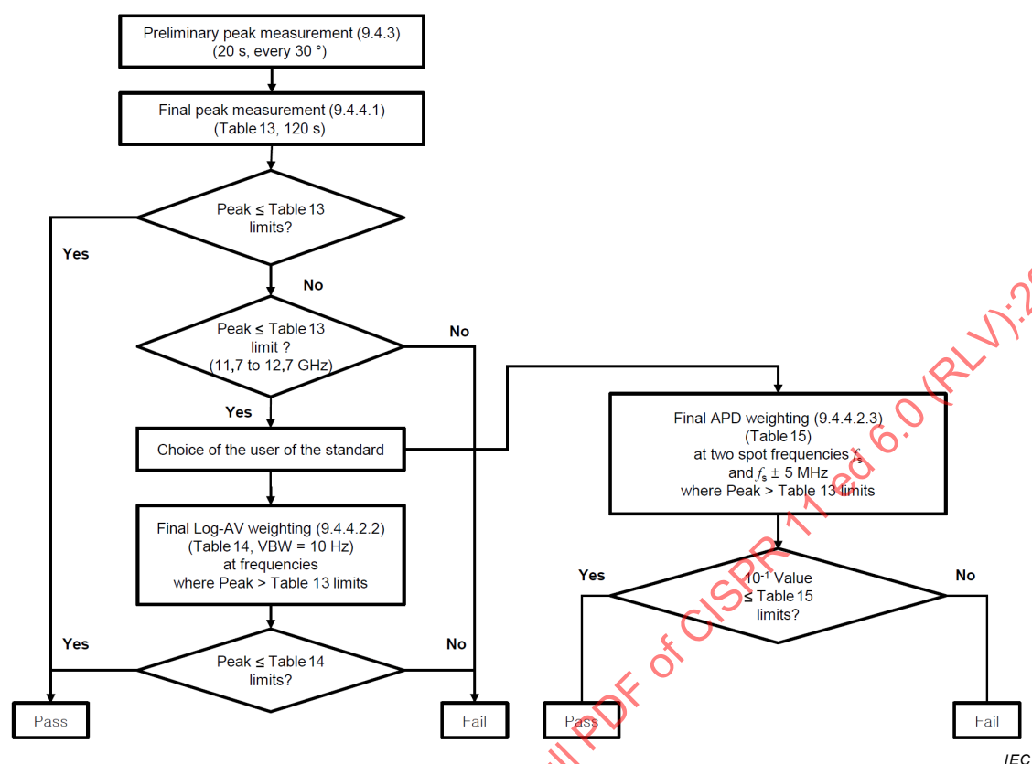
Figure 5 12 – Decision tree for the measurement of emissions from 1 GHz to 18 GHz of class B, group 2-ISM equipment operating at frequencies above 400 MHz
