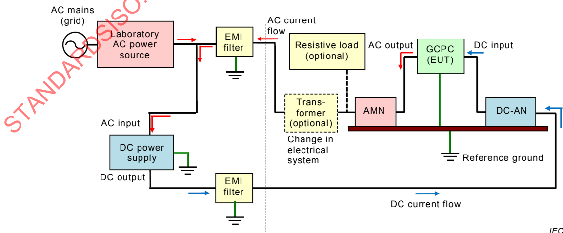
Figure J.1 – Setup of the test site (Case 1) – 2D diagram
