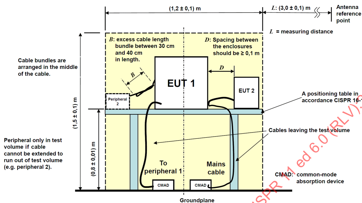
Figure 3b – Side view
