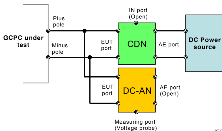
Figure 7 – Typical arrangement for measurement of conducted disturbances at LV d.c. power ports with the DC-AN used as termination and voltage probe
