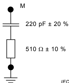
Figure 6 2 – Artificial hand, RC element (see 7.3.5)
