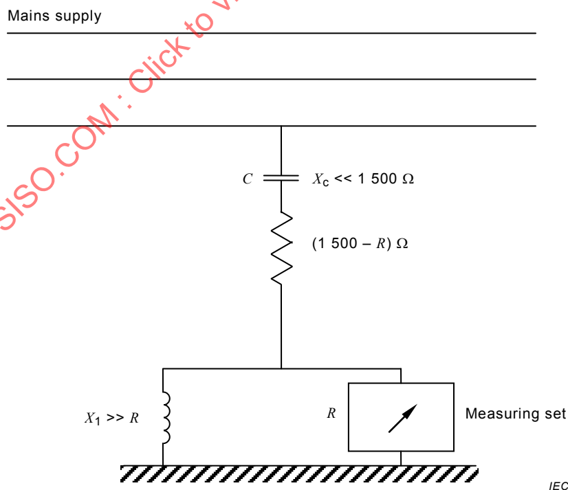
Figure 4 1 – Circuit for disturbance voltage measurements on mains supply (see 7.3.3)
