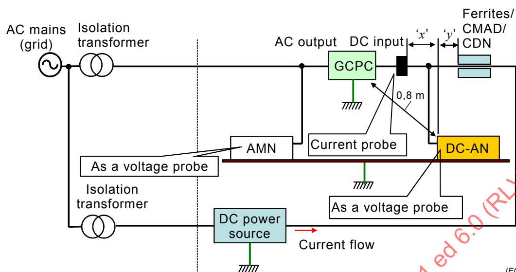
Figure 8 – Typical arrangement for measurement of conducted disturbances at LV d.c. power ports with the DC-AN used as voltage probe and with a current probe – 2D diagram
