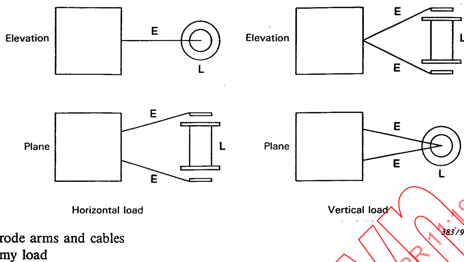
Fig. 3 — Disposition of medical apparatus (capacitive type) and dummy load (see 7.5.1.1).
