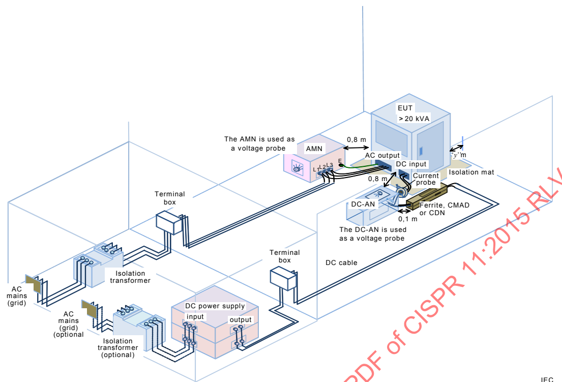
Figure 9 – Typical arrangement for measurement of conducted disturbances at LV d.c. power ports with a DC-AN used as voltage probe and with a current probe – 3D diagram
