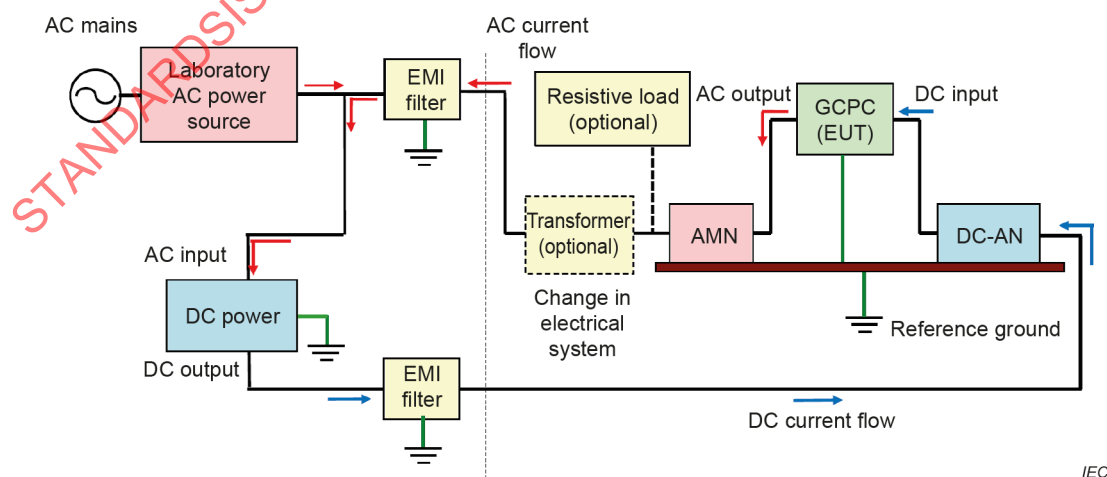
Figure D.1 – Setup of the test site (Case 1) – 2D diagram Test setup for Case 1 (schematic)
