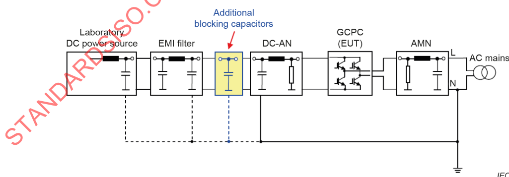
Figure E.3 – Blocking of flow of common mode RF current by employment of additional CM decoupling capacitors
