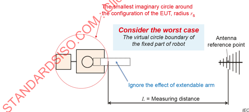
Figure 5 – EUT boundary determination for radiated disturbance measurements of robots with extendable/moving arm
