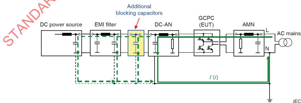
Figure E.5 – Prevention of saturation of mitigation filters by use of additional decoupling capacitors
