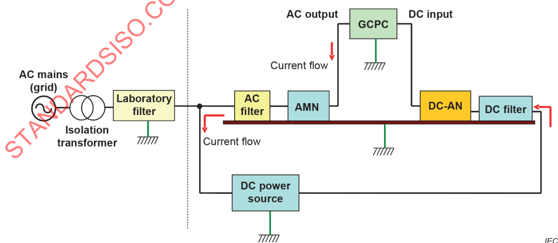
Figure 11 – Typical arrangement for measurement of conducted disturbances at LV DC power ports with the DC-AN used as termination and decoupling unit to the laboratory DC power source
