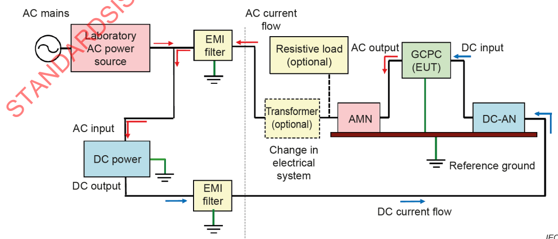
Figure D.1 – Test setup for Case 1 (schematic)
