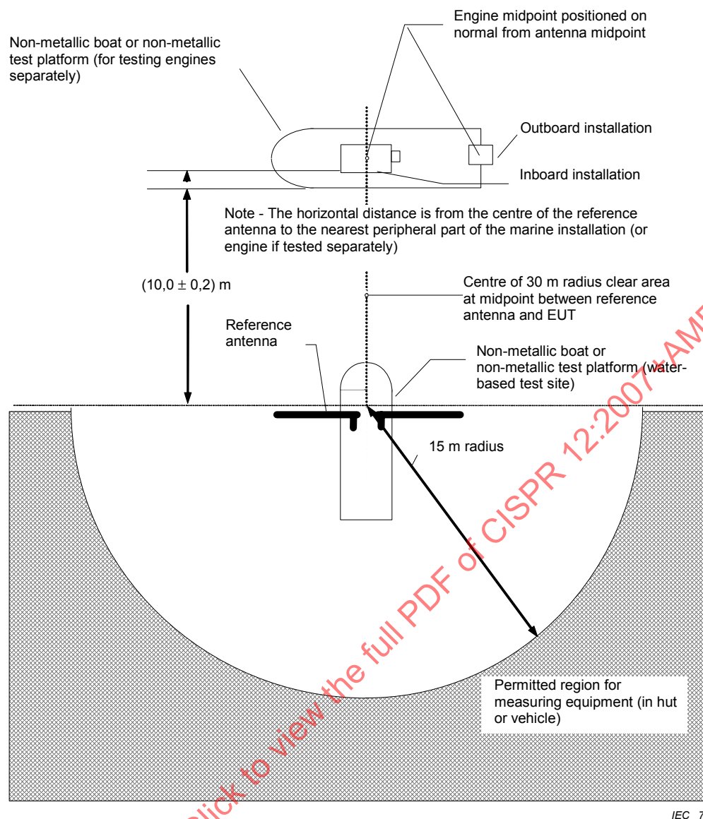
Figure 5 – Measuring site (OTS) for boats
