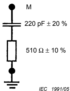
Figure 8a – RC element
