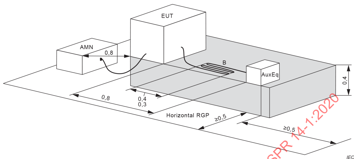
Figure 23 – Example of test setup for disturbance voltage measurements on table-top EUT (horizontal RGP)
