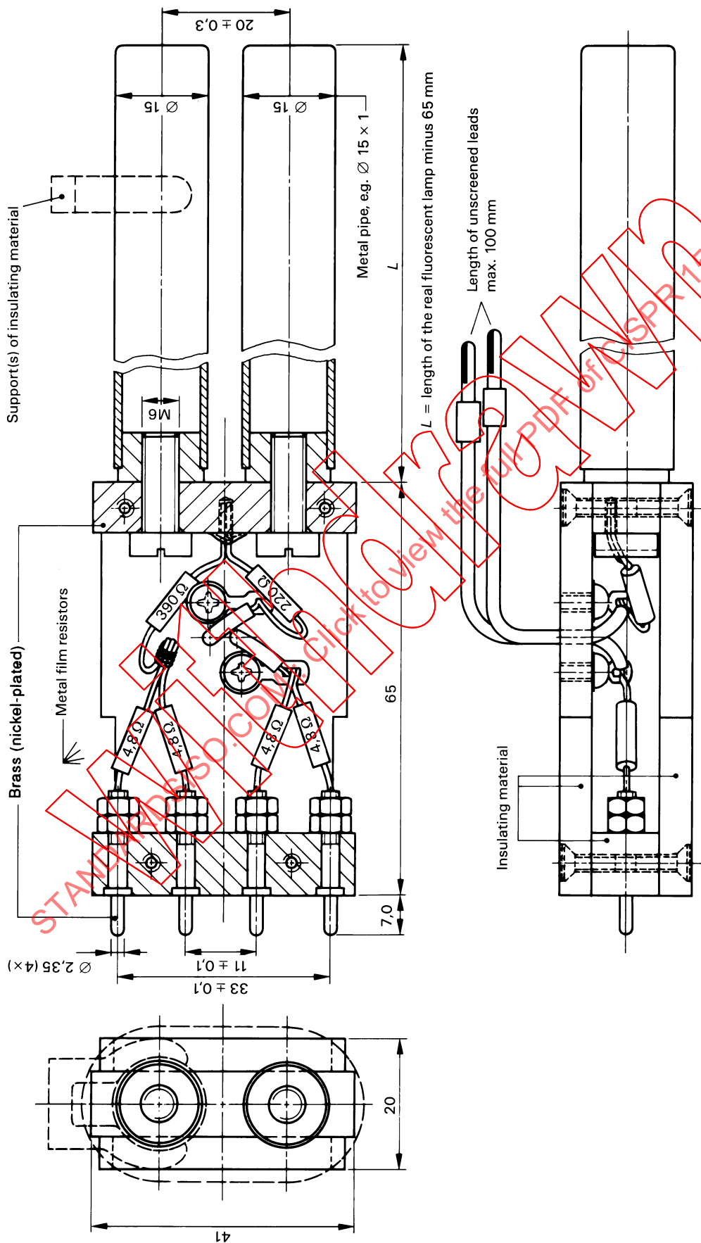
IEC 1365/2000 Dimensions in millimetres Figure 4d – Dummy lamp for 15 mm single-capped fluorescent lamps
