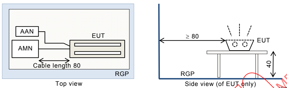
Figure 8a – Horizontal RGP setup (option 1)
