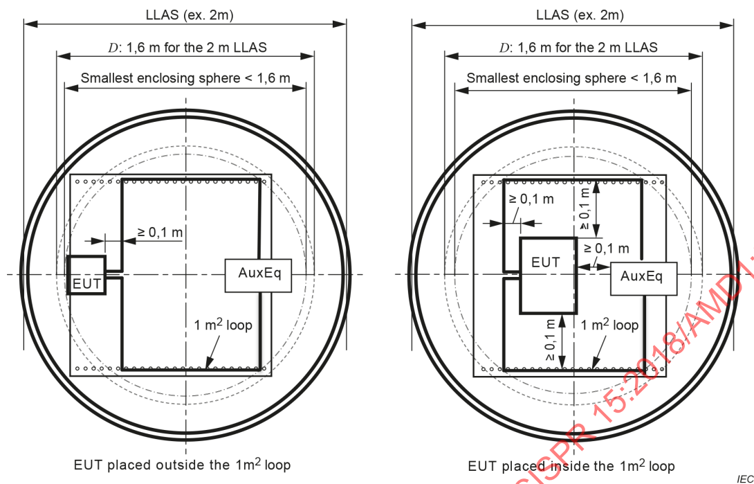
Figure C.6a – Top view
