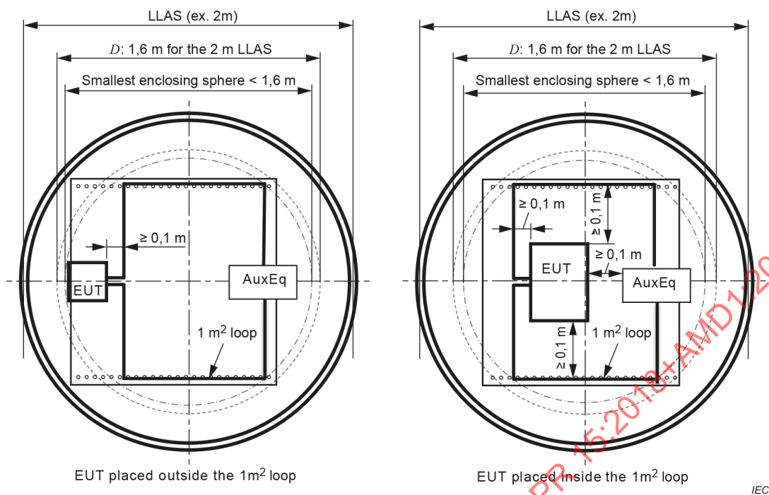
Figure C.6a – Top view
