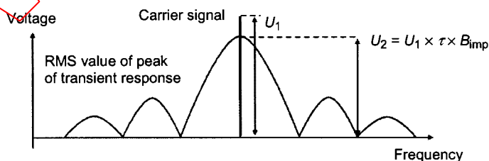
Figure E.6– Filtering with a B_{\text{imp}} much wider than the prf
