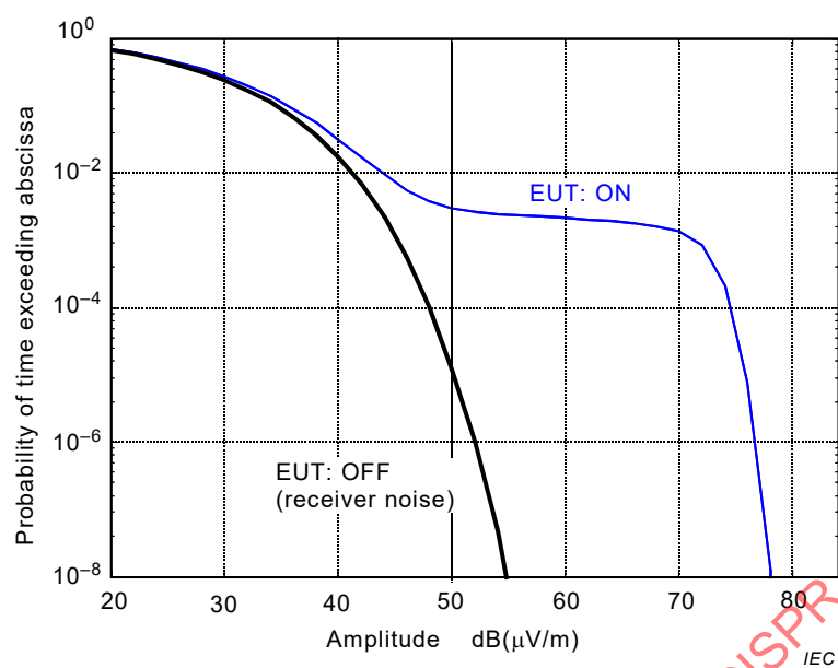
Figure G.3 – Example of display of APD measurement results versus equipment-under-test (EUT) state
