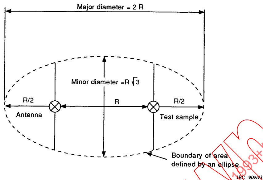
Figure 14 – Obstruction-free area of a test site with a turntable. (Subclause 16.3)
