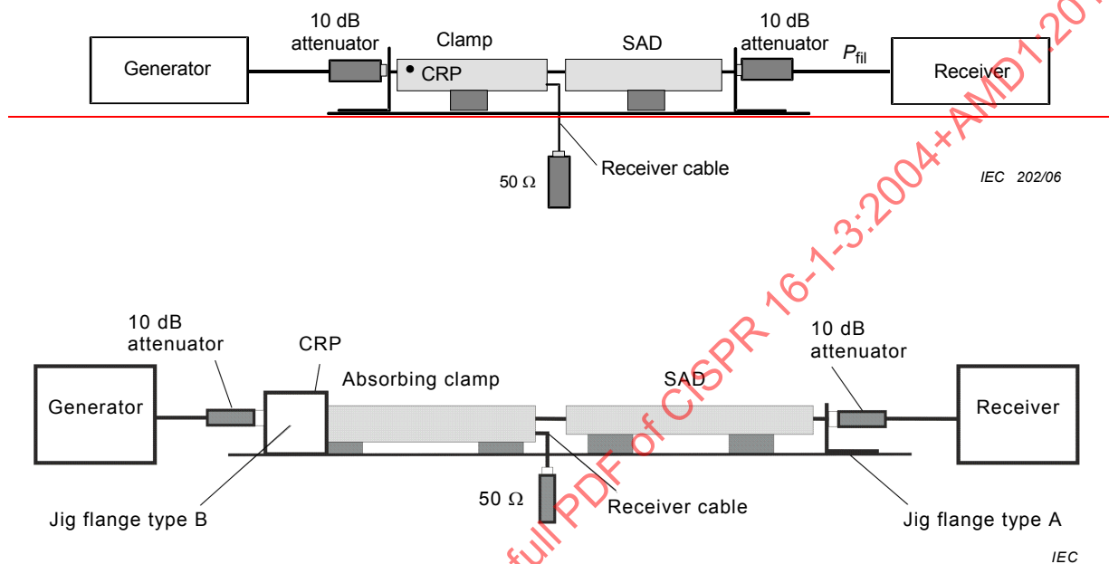
Figure B.8b – Measurement with the absorbing clamp and SAD placed in the jig
