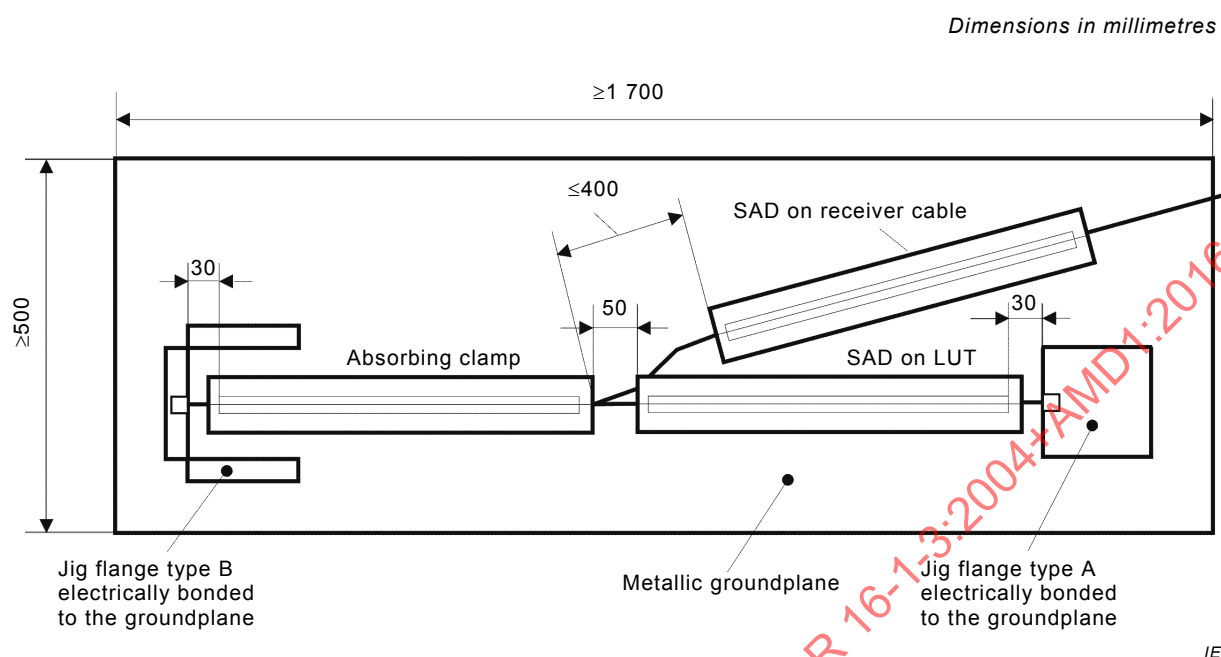
Figure B.4 – Top view of the jig
