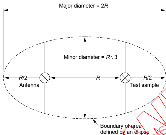
Figure 2 – Obstruction-free area of a test site with a turntable (see 5.3)
