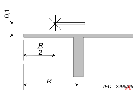
Figure 12 – Antenna position above the set-up table (side view)
