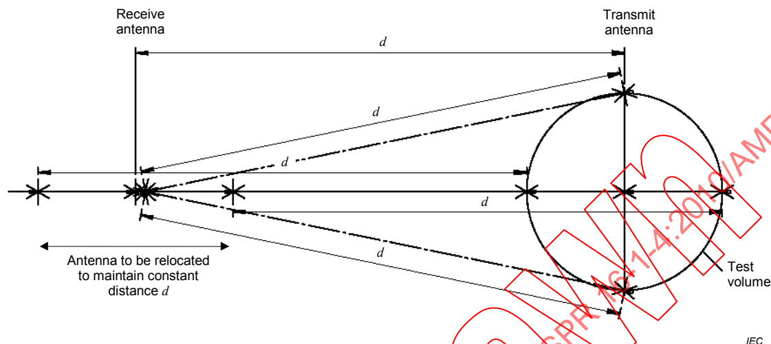
Figure 35 – Typical antenna positions for a weather-protected OATS or a SAC – Vertical polarization validation measurements
