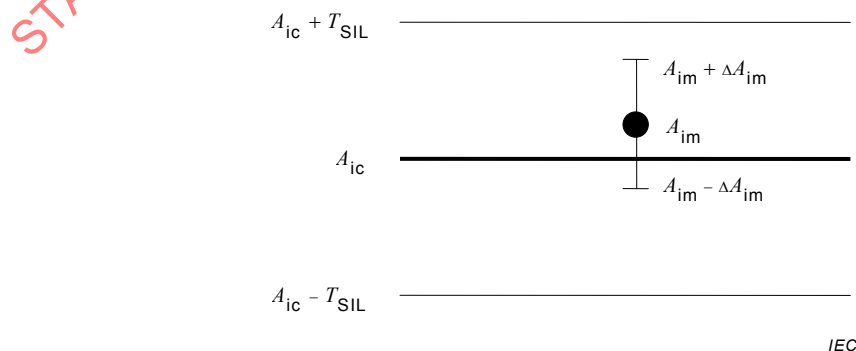
Figure 7 – Relation between the quantities used in the SIL acceptance criterion
