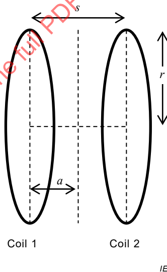
Figure H.1 – Diagram of Helmholtz coil method set-up
