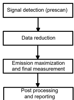
Figure 24 – Process to give reduction of measurement time
