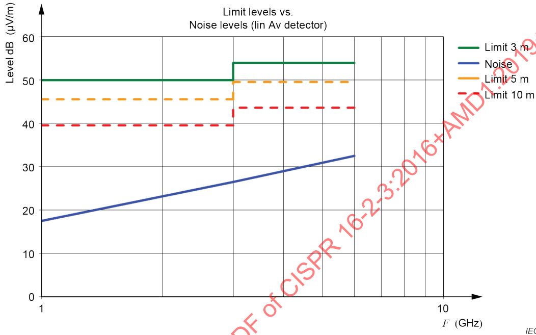
Figure F.7 – Noise level E_{N\text{linav}} (example for 10\lg F_{\text{tot}} = 4 dB) compared with the disturbance limit E_{L\text{av}} for the linear average detector for 3 m, 5 m, and 10 m distances in the frequency range 1 GHz to 6 GHz
