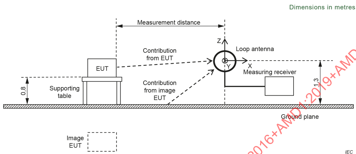
Figure 25 – Concept of magnetic field strength measurement set-up at an OATS or in a SAC for table-top EUT
