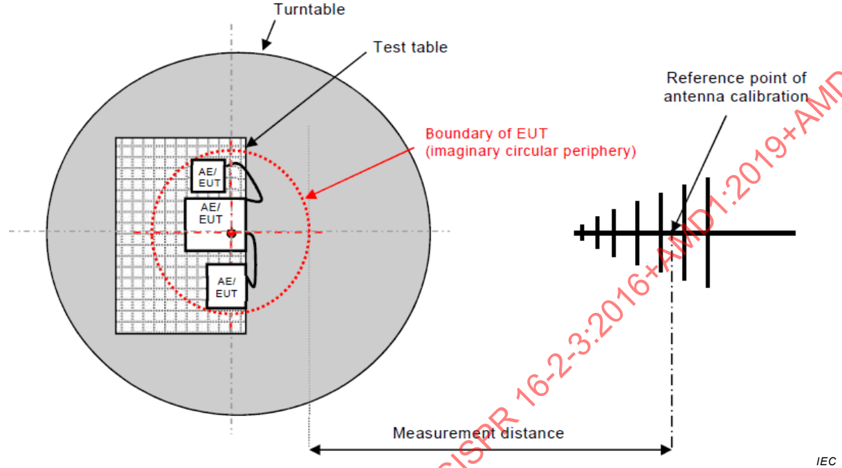
Figure 8 – Measurement distance
