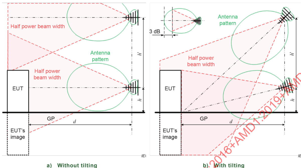
Figure F.4 – Effect of antenna directivity
