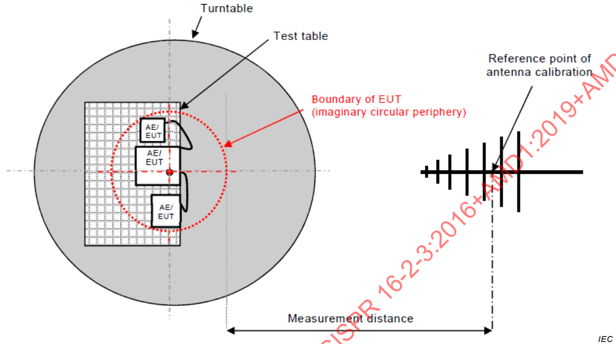
Figure 8 – Measurement distance
