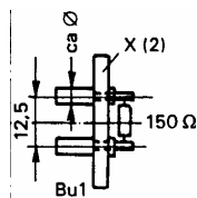
Figure E.6 – Terminating impedance TI
