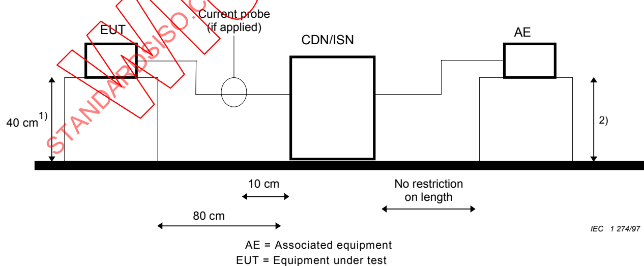
Figure C.1 – Using CDNs described in IEC 61000-4-6 as CDN/ISNs
