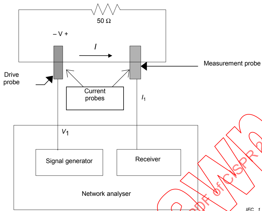
Figure C.5 – Calibration fixture
