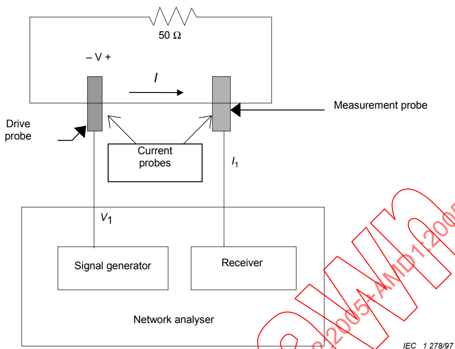
Figure C.5 – Calibration fixture
