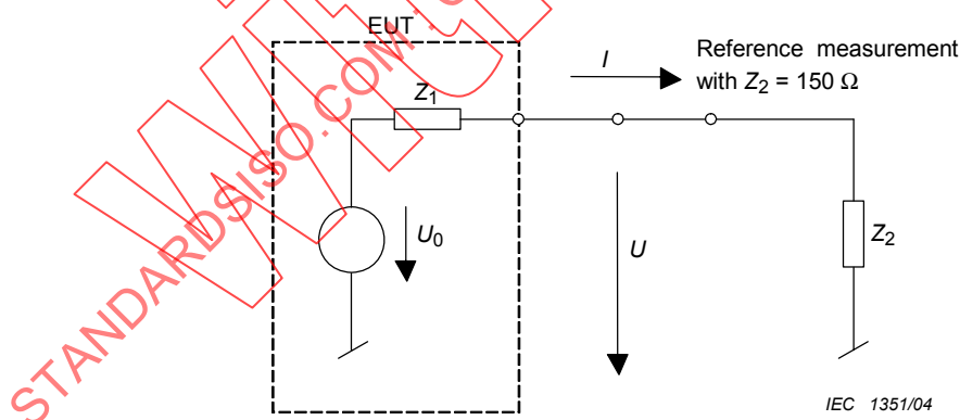
Figure F.1 – Basic circuit for considering the limits with defined TCM impedance of 150\ \Omega
