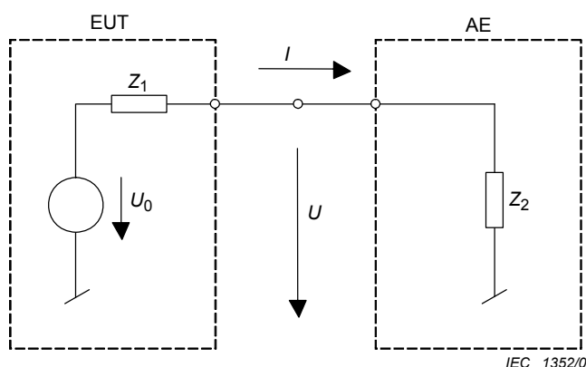
Figure F.2 – Basic circuit for the measurement with unknown TCM impedance
