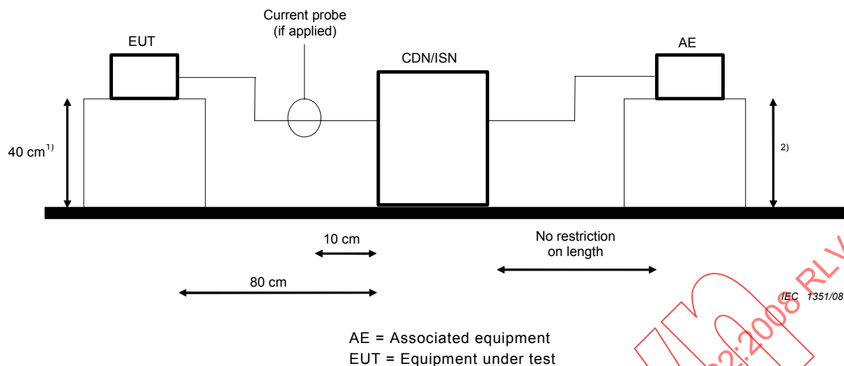
Figure C.1 – Using CDNs described in IEC 61000-4-6 as CDN/ISNs
