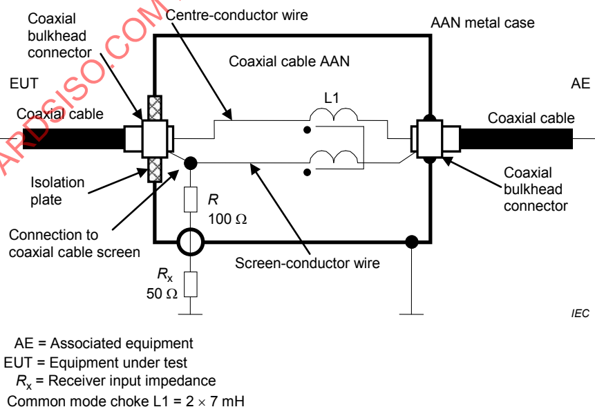
Figure G.7 – Example AAN for use with four unscreened balanced pairs
