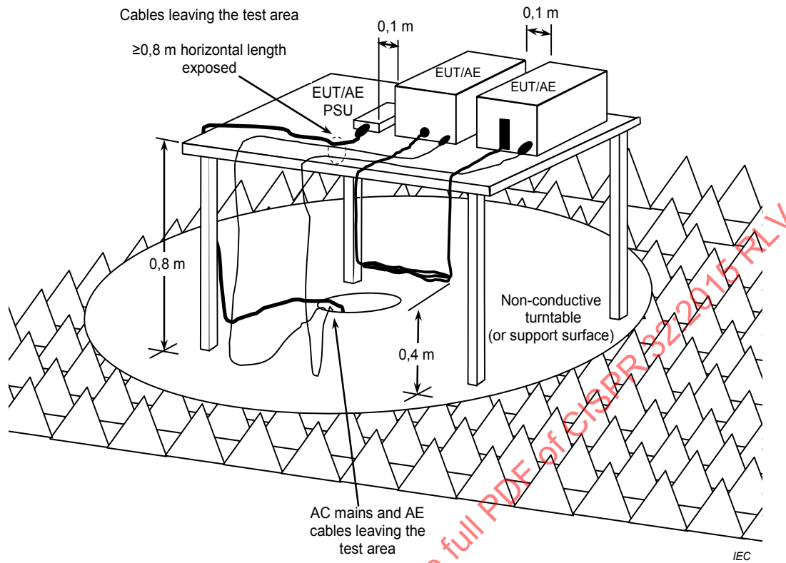
Figure D.11 – Example measurement arrangement for tabletop EUT (radiated emission measurement within a FAR)
