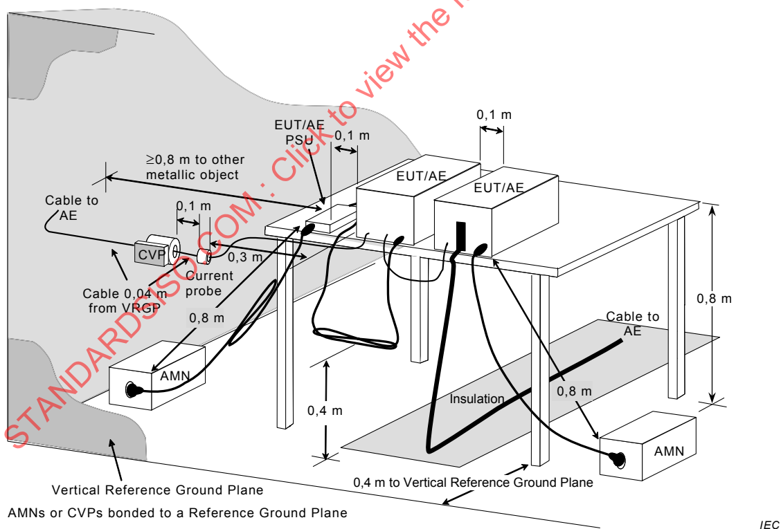
Figure D.3 – Example measurement arrangement for table-top EUT (conducted emission measurement – alternative 2)
