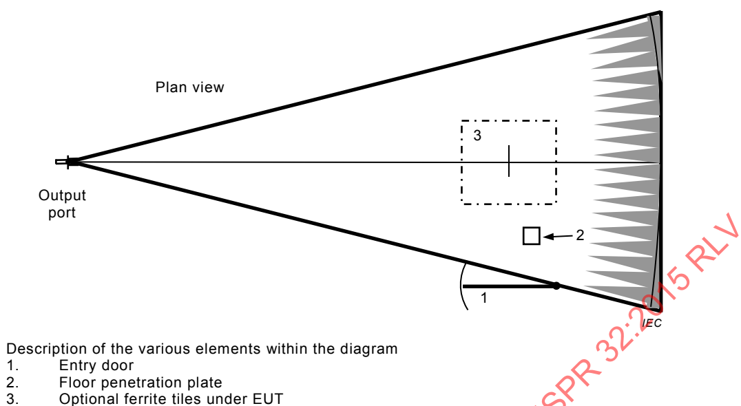
Figure I.2 – Typical GTEM plan sectional view showing floor layout
