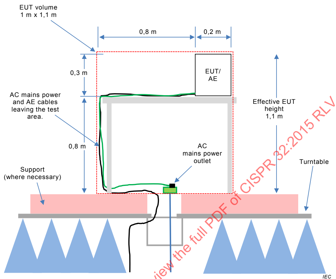
Figure D.12 – Example cable configuration and EUT height (radiated emission measurement within a FAR)
