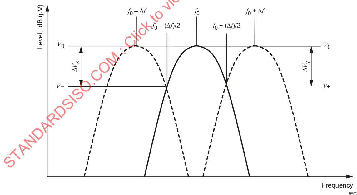
Figure B.1 – Example of measurement for frequency step uncertainty evaluation
