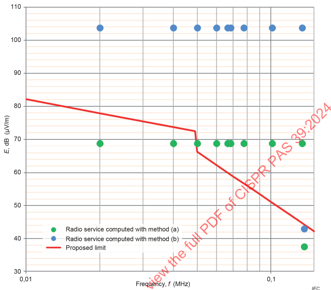
Figure A.5 – Proposed field strengths limits compared to protection needs of radio applications
