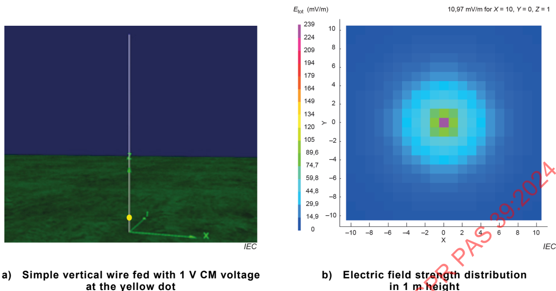
Figure A.2 – Worst case common mode radiator for residential environment
