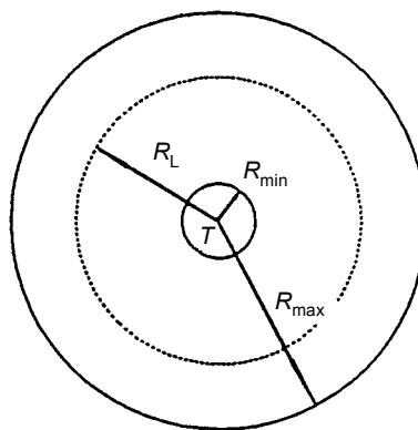
Figure 4.4-A1 – Definition of the ring-shaped area round the transmitter T
