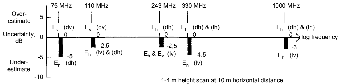
Figure 4.5-18 – Ranges of uncertainties in the predictability of radiation in vertical directions from electrically small sources located at a height of 1 m or 2 m above ground. The predictability is based on measurements of the horizontally and vertically polarized E -fields in a height scan from 1 m to 4 m at a horizontal distance of 10 m from the sources. The following example shows how the bar chart can be interpreted. At 243 MHz, the bar shows that the best predictability, with nominally zero error, is obtained when estimating the maximum strength of the horizontally polarized E_h field emitted at elevated angles from a source behaving as a small horizontal dipole (dh). The poorest predictability at 243 MHz, an underestimate by as much as 2,5 dB, can occur when predicting the maximum strengths of the horizontally polarized E_h fields and the E_z vertical component of the vertically polarized fields emitted at elevated angles from a source behaving as a small vertical loop (lv). (Reproduced from [10])
