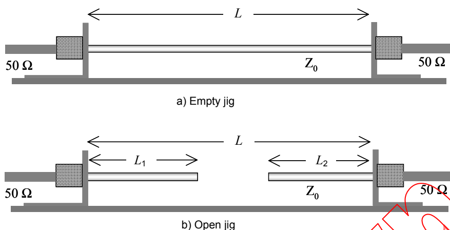
Figure 179 – Preliminary measurements of the test set-up
