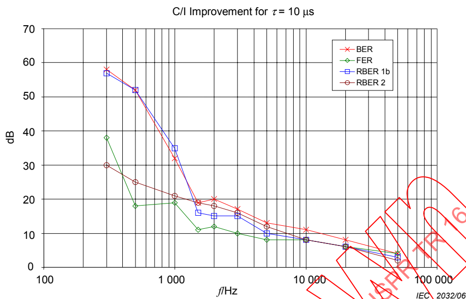
Figure 160 – Carrier-to-interference improvements with decreasing PRF in dB computed for GSM using COSSAP
