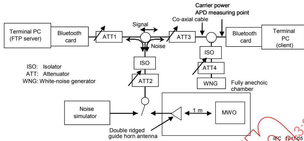
Figure 116 – Set-up for measuring the communication quality degradation of Bluetooth
