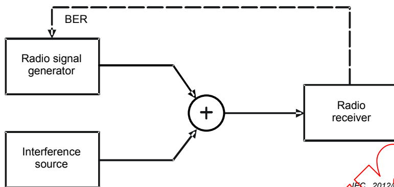
Figure 142 – Test setup for the measurement of the pulse weighting characteristics of a digital radiocommunication system
