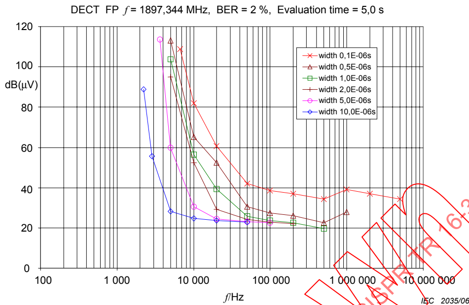
Figure 163 – Weighting characteristics for DECT (signal level –83 dBm)
