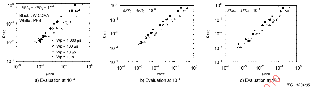
Figure 139 – Correlation between measured p_{BER} and p_{APD}
