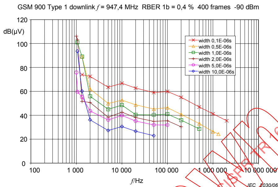
Figure 158 – Weighting characteristics for RBER 1b of GSM (signal level -90 dBm)
