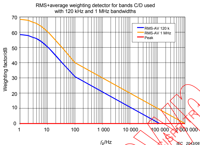
Figure 171 – Shift of the rms-average weighting function for CISPR band C/D by using a bandwidth of 1 MHz instead of 120 kHz, if the shortest possible pulse widths are applied
