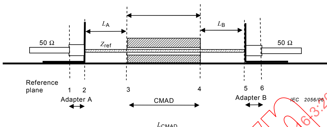
Figure 180 – Position of the reference planes for the measurement with SOLT calibration and ABCD transformation to Z_{ref} level
