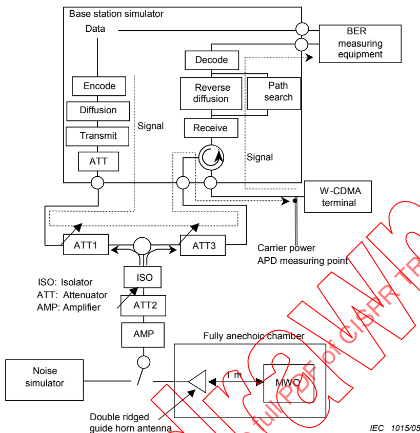
Figure 120 – Set-up for measuring the BER of W-CDMA
