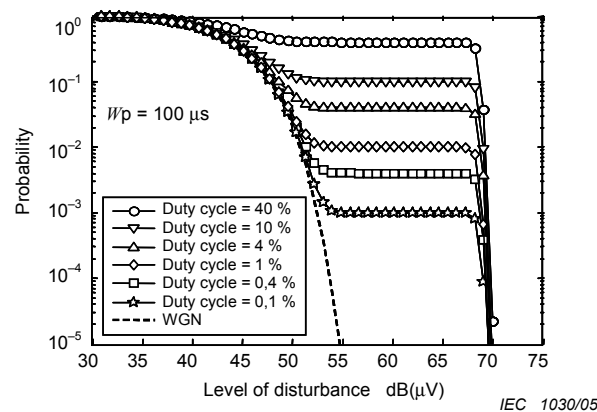
Figure 135 – APD of pulse disturbance
