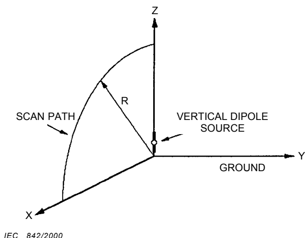
Figure 51 – Geometry of the small vertical electric dipole model
