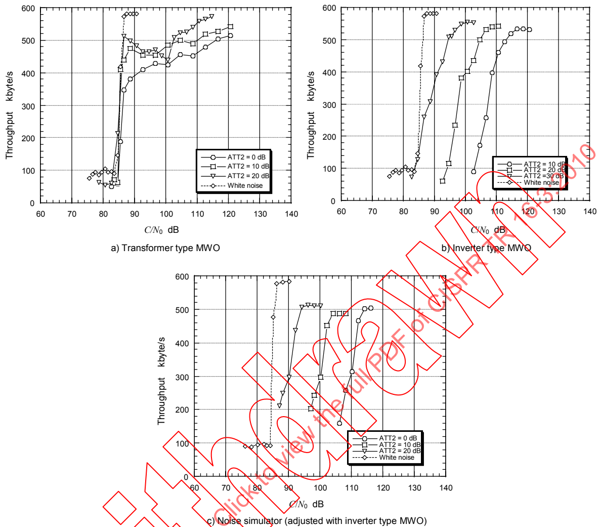
Figure 115 – Wireless LAN throughput influenced by noise
