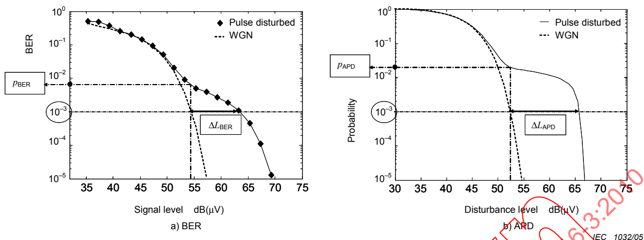
Figure 137 – Evaluation method of the correlation between BER and APD
