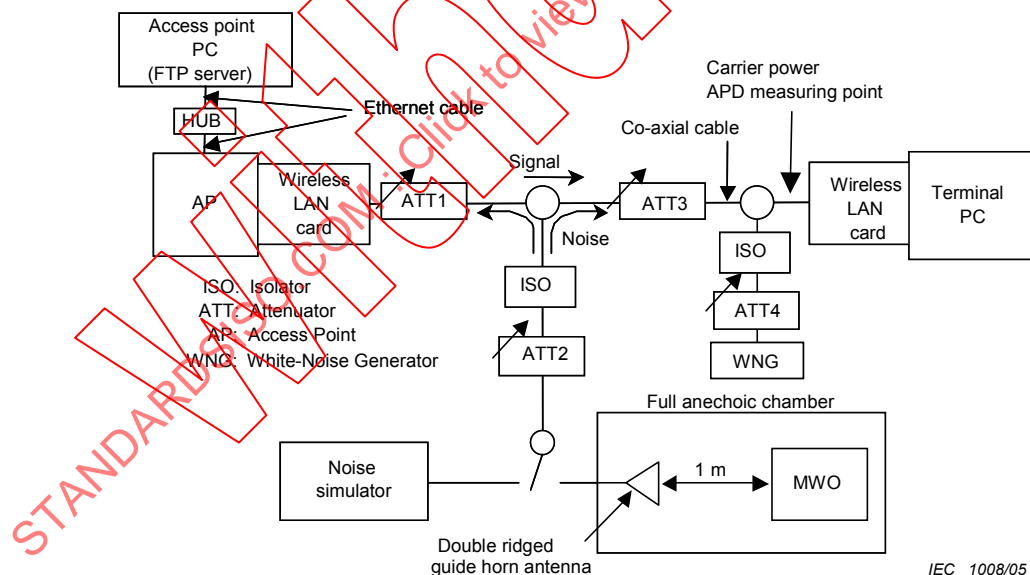
Figure 113 – Set-up for measuring communication quality degradation of a wireless LAN
