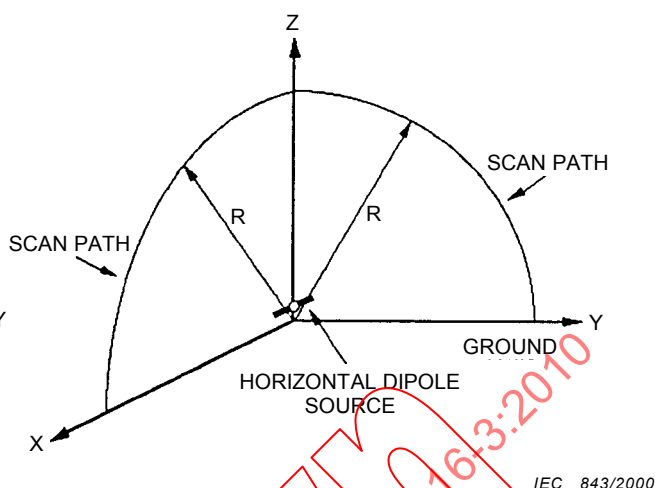
Figure 52 – Geometry of the small horizontal electrical dipole model
