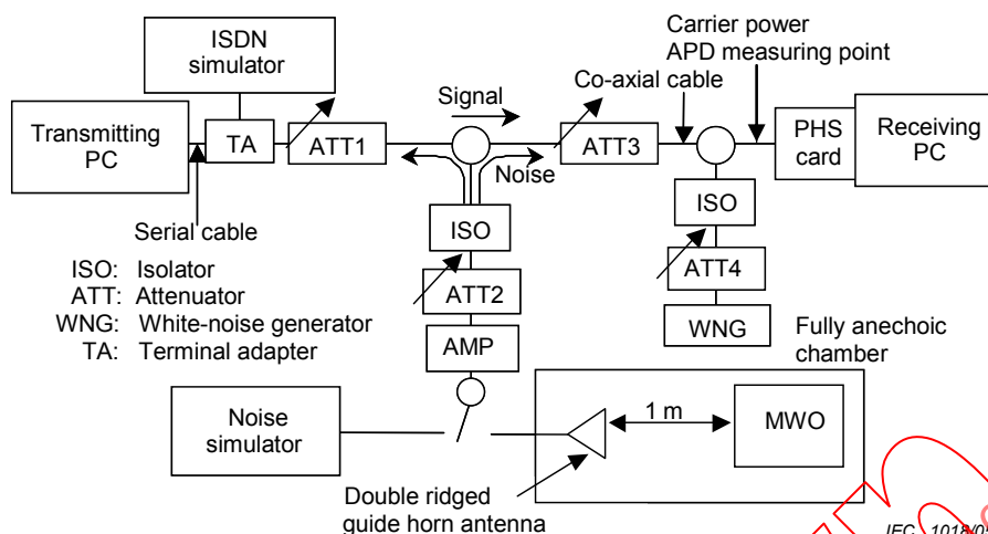
Figure 123 – Set-up for measuring the PHS throughput
