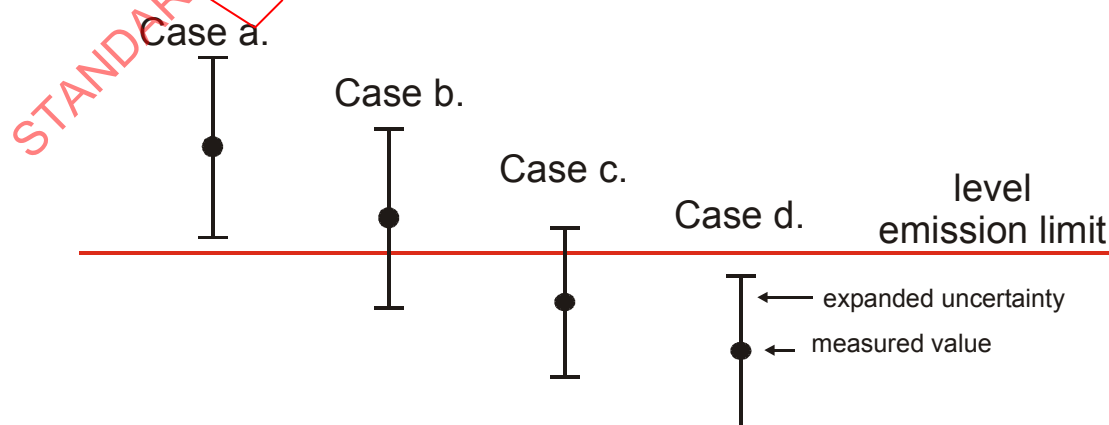
Figure 8 – Graphical representation of four cases in the compliance determination process.
