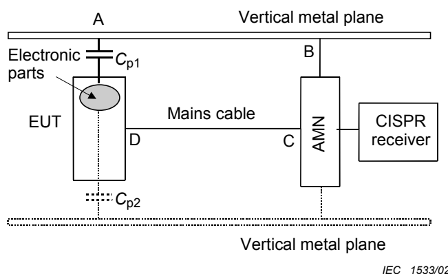
Figure 6-7 – Variation of the parasitic capacitance, and hence of the CM-impedance, by changing the position of the reference plane (non-conducting EUT housing)
