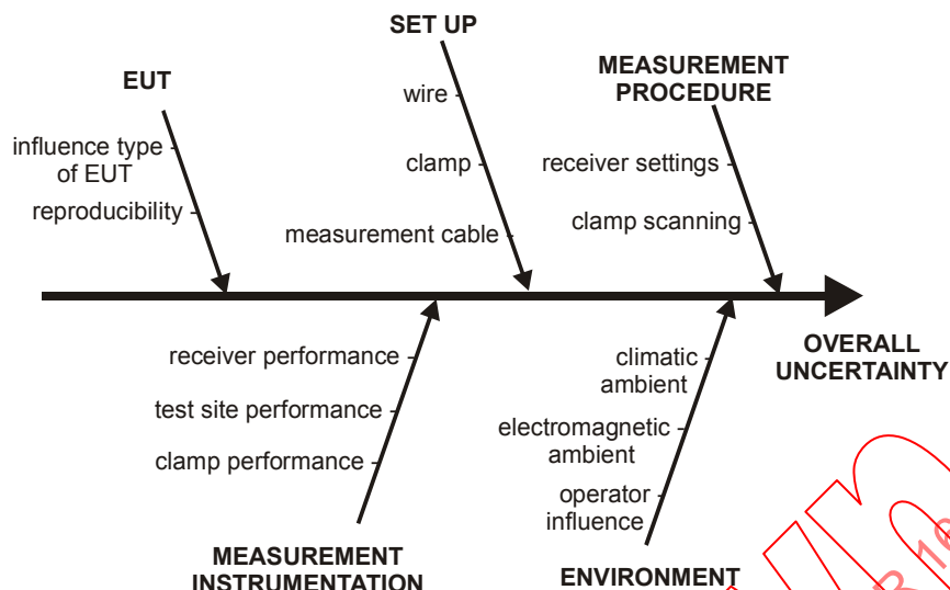
Figure 6 – Example of a fishbone diagram indicating the various uncertainty sources for an absorbing clamp compliance measurement in accordance with CISPR 16-2
