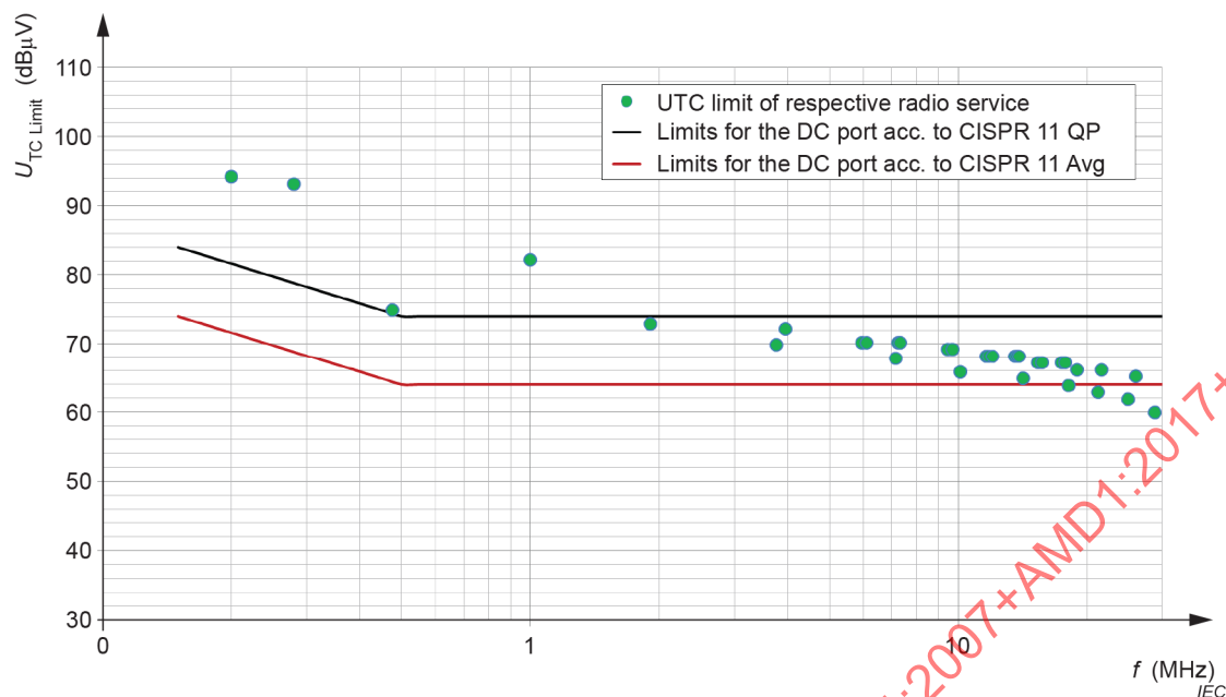
Figure C.24 – Overview of the calculated U_{TC\ Limit} values for radio services between 150 kHz and 30 MHz at a distance of d = 10 \text{ m}
