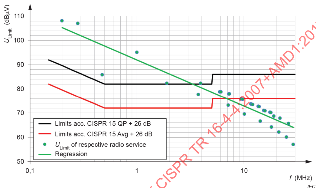
Figure D.9 – Overview of the calculated U_{Limit} values for radio services between 150 kHz and 30 MHz
