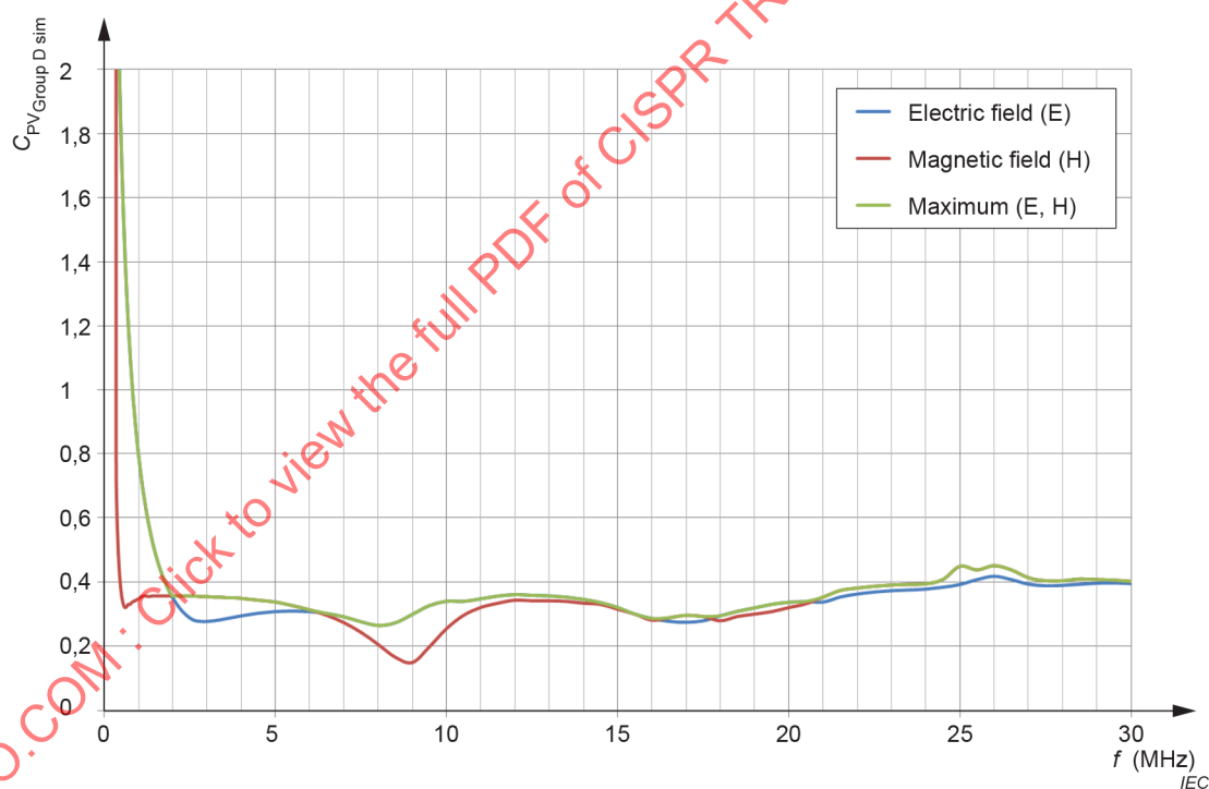
Figure C.14 – Combined coupling factor C_{PV \text{ Group D sim}} for Group D PV generators ( r = 10 \text{ m} )
