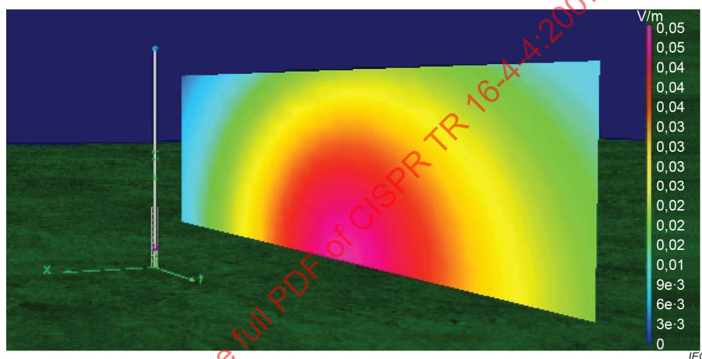
b) Capacitive load distance to wires 5 cm
