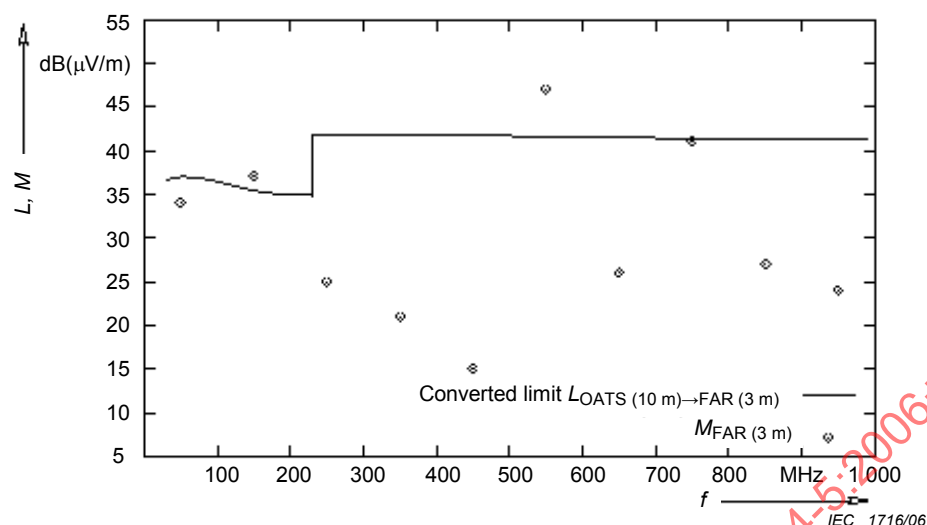
Figure B.15 – Comparison of the measured values with the corrected converted limit
