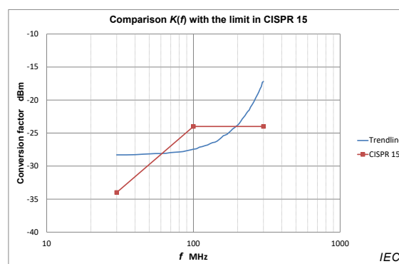
Figure C.7 – Comparison with CISPR 15:2013
