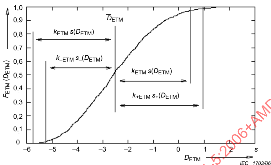
Figure B.6 – Sample cumulative distribution function
