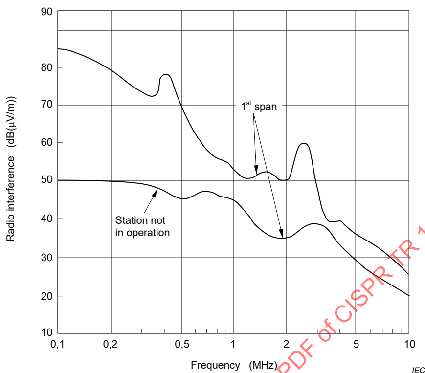
Figure 19 – Example of frequency spectra of the radio interference in the vicinity of an AC line (20 m) at a short distance from the converter station
