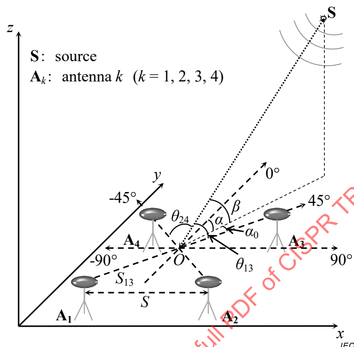
Figure B.2 – Coordinates and arrangement of the four-antenna-square array
