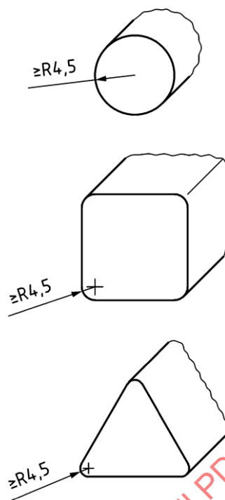
Figure 4 — Rounding of parts
