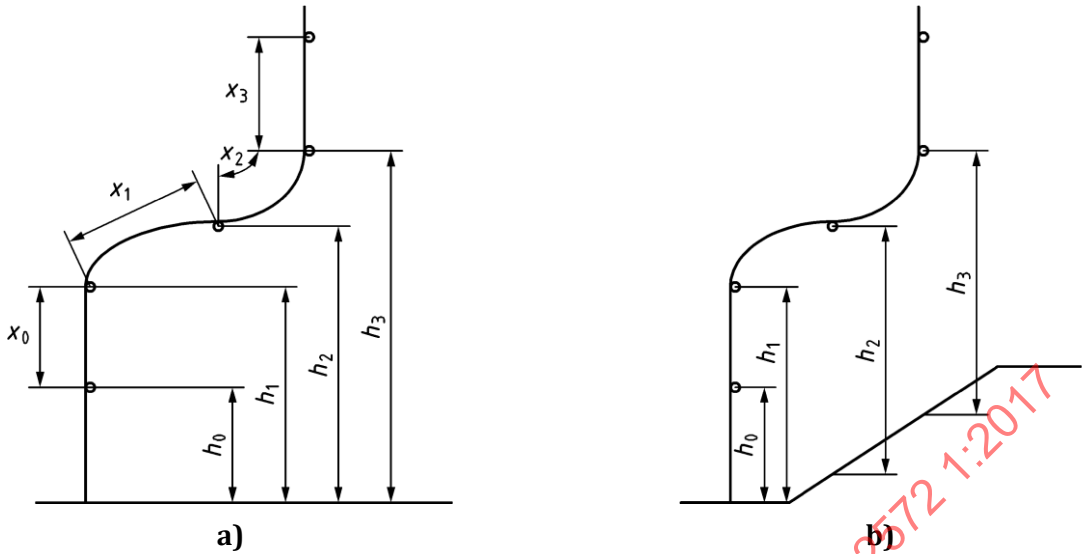
Figure 1 — Layout of protection points
