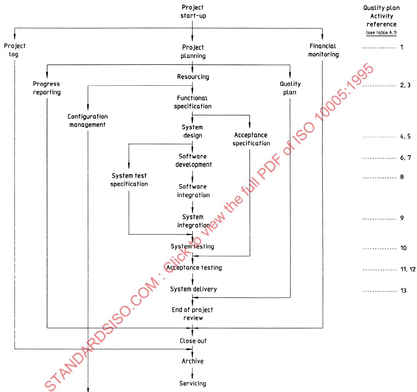
Figure A.4 — Simplified example of a software life cycle
