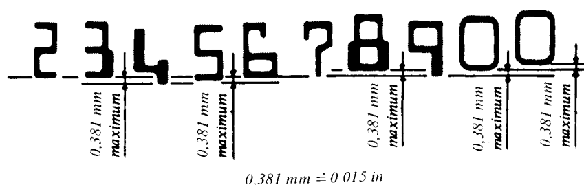
FIGURE 17 – Allowable variation in vertical alignment
