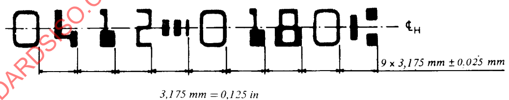
FIGURE 16 — Distance between characters
