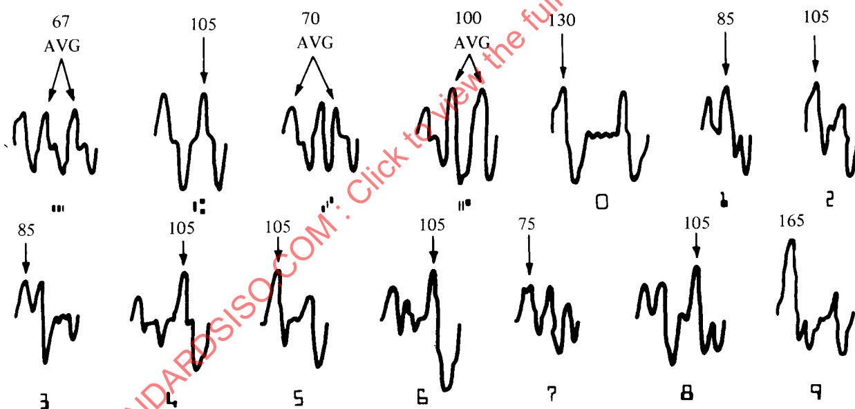
FIGURE 27 — Wave form peaks for signal level measurement
