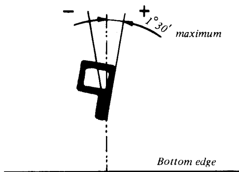
FIGURE 18 — Allowable character skew
