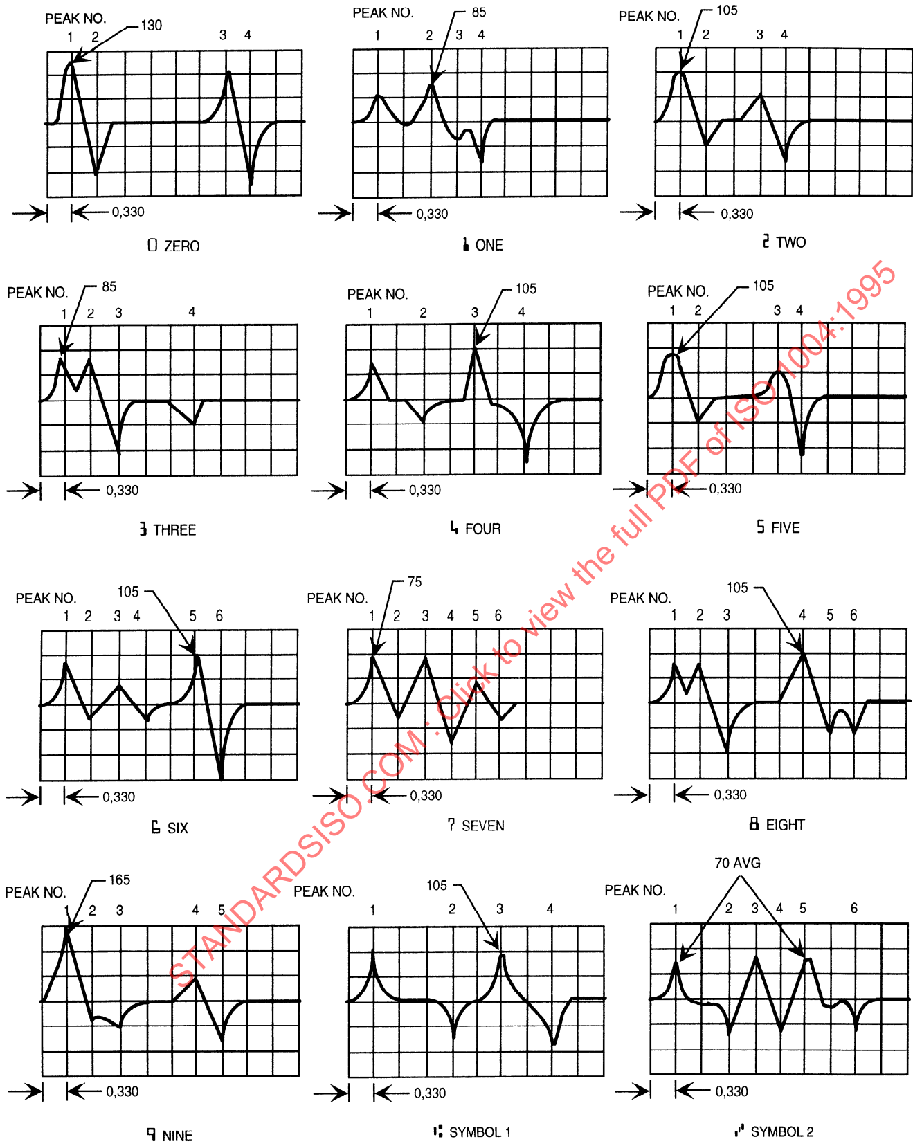
Figure 27 — Ideal waveform peaks
