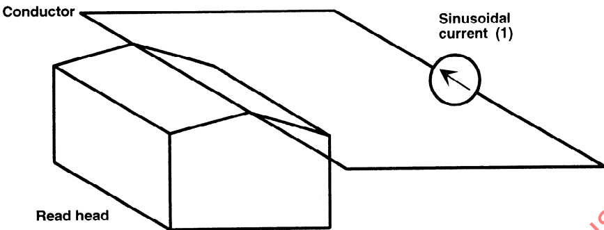
Figure 29 — Conductor arrangement for wire card calibration method
