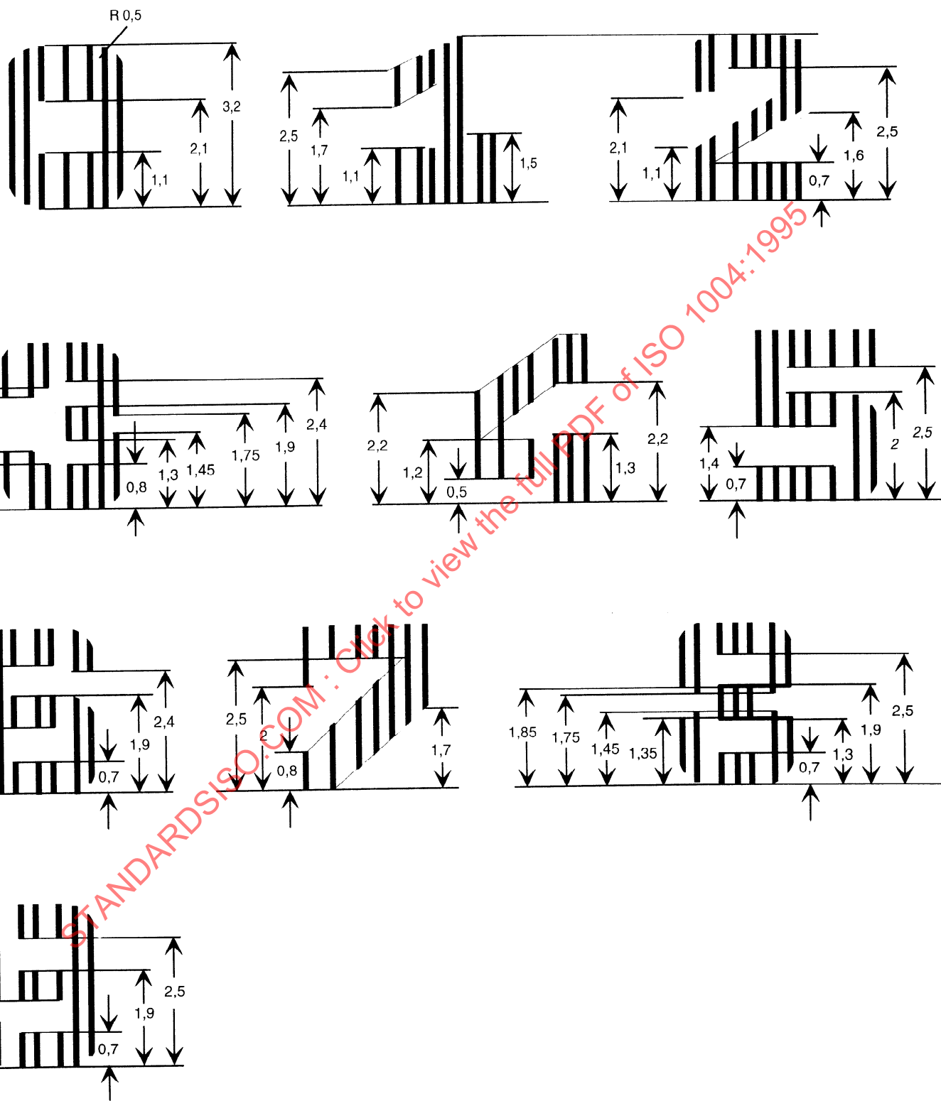
Figure 34 — Digits: Font height 3,20 mm ( H_t )
