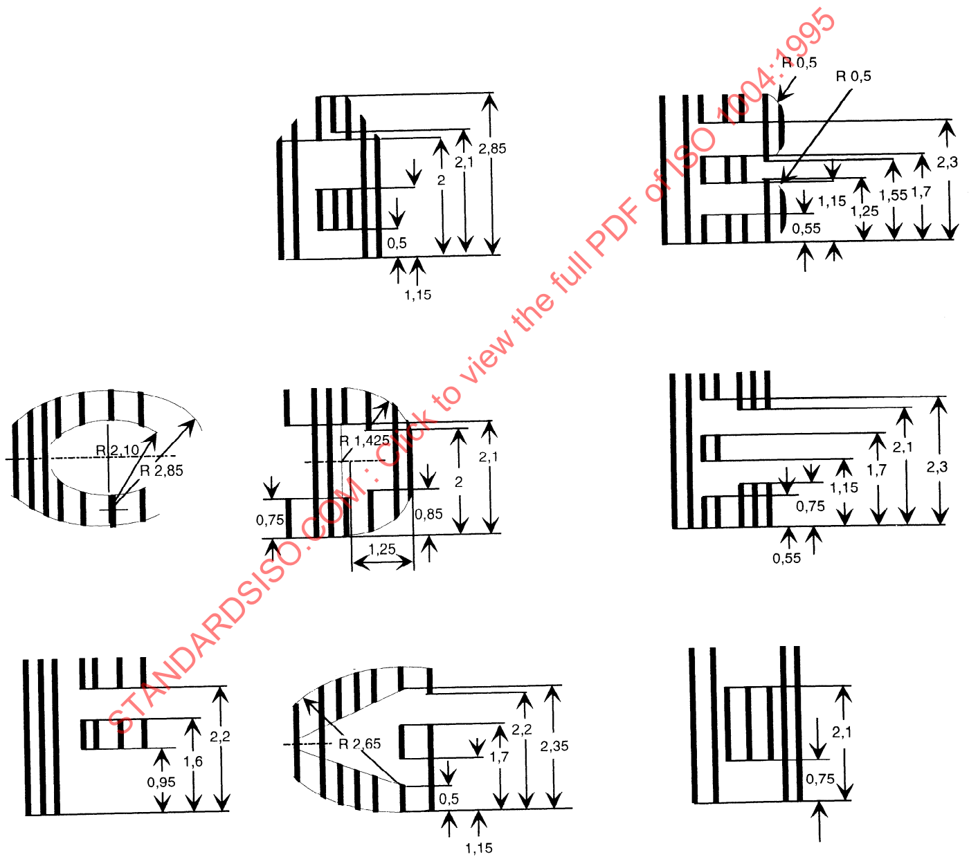
Figure 46 — Letters A to H: Font height 2.85 mm ( H_{13} )
