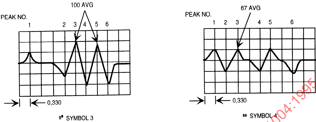
Figure 27 — Ideal waveform peaks (concluded)
