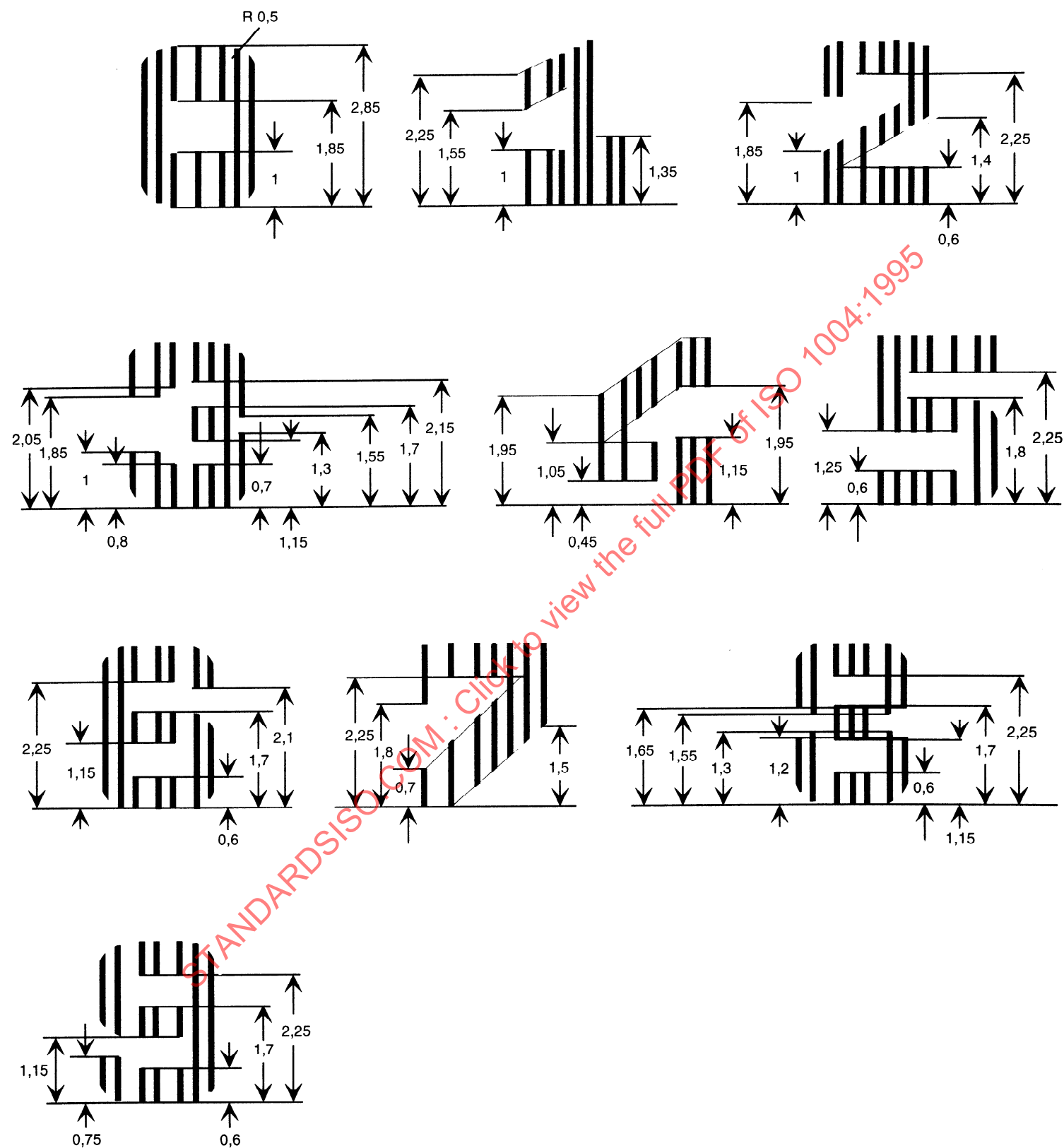
Figure 44 — Digits: Font height 2,85 mm ( H_{13} )
