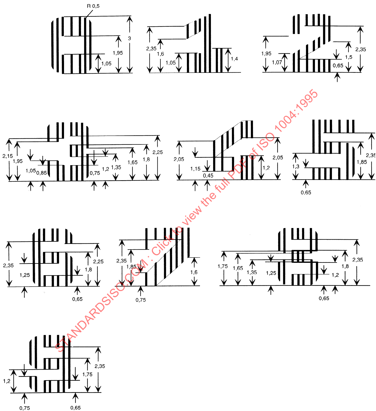
Figure 39 — Digits: Font height 3,00 mm ( H_{12} )
