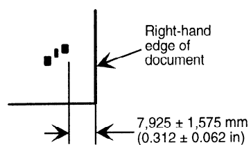
Figure 31 - Distance of the right hand character from the right hand reference edge
