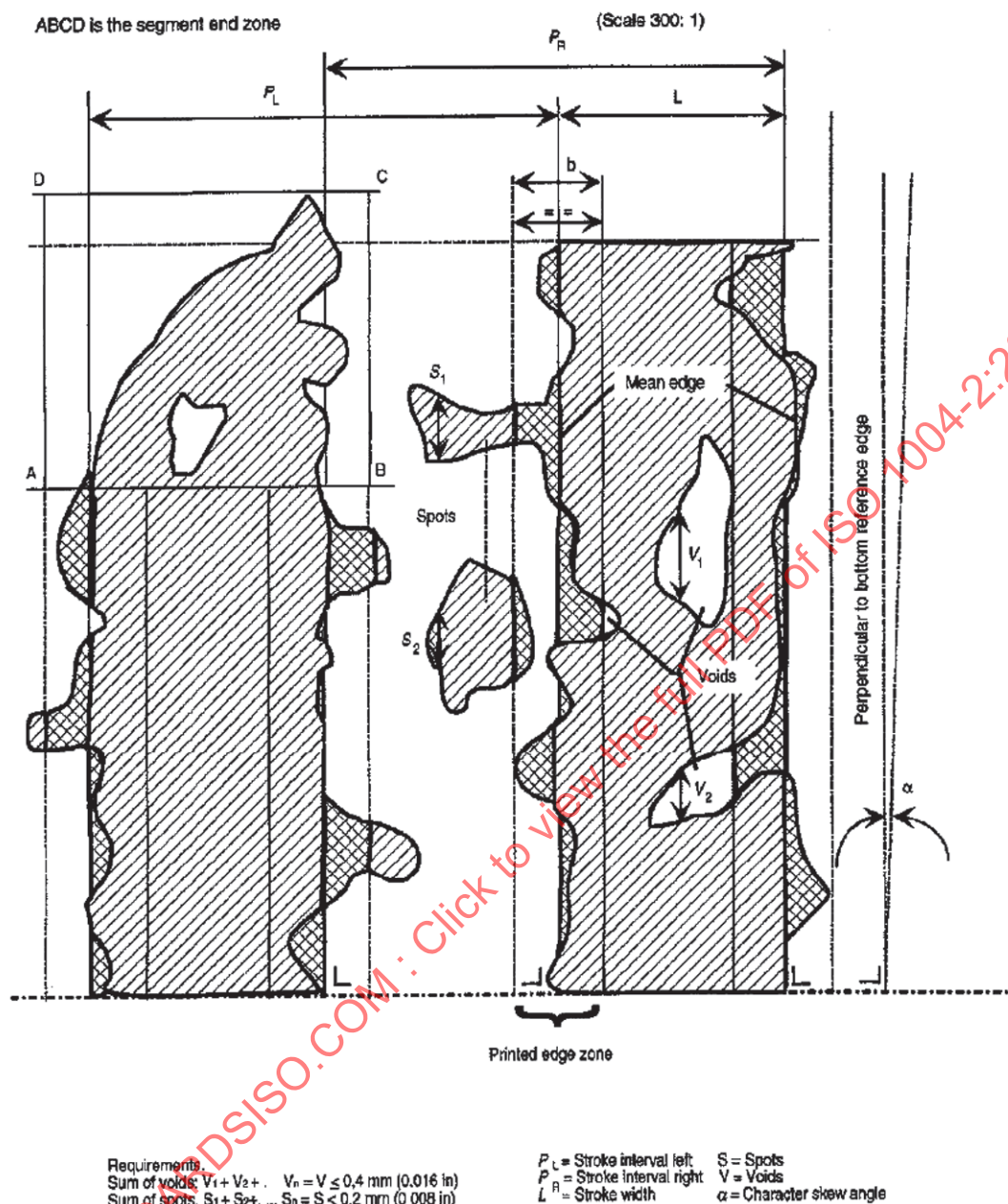
Figure 2 — Magnified view of part of a character
