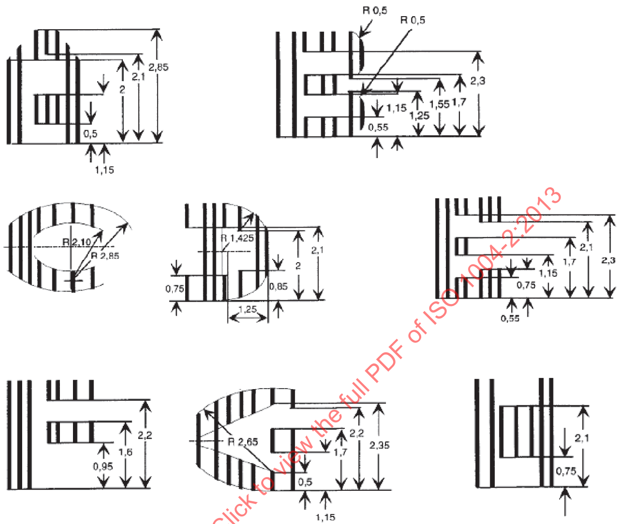
Figure 15— Letters A to H: Font height 2,85 mm ( H_{13} )
