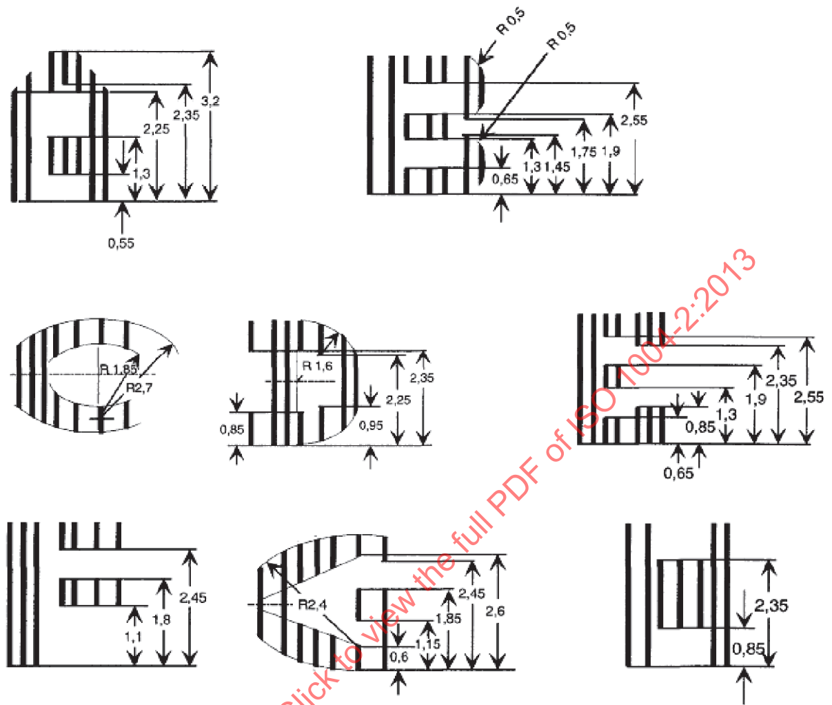
Figure 5 — Letters A to H: Font height 3,20 mm ( H_{11} )
