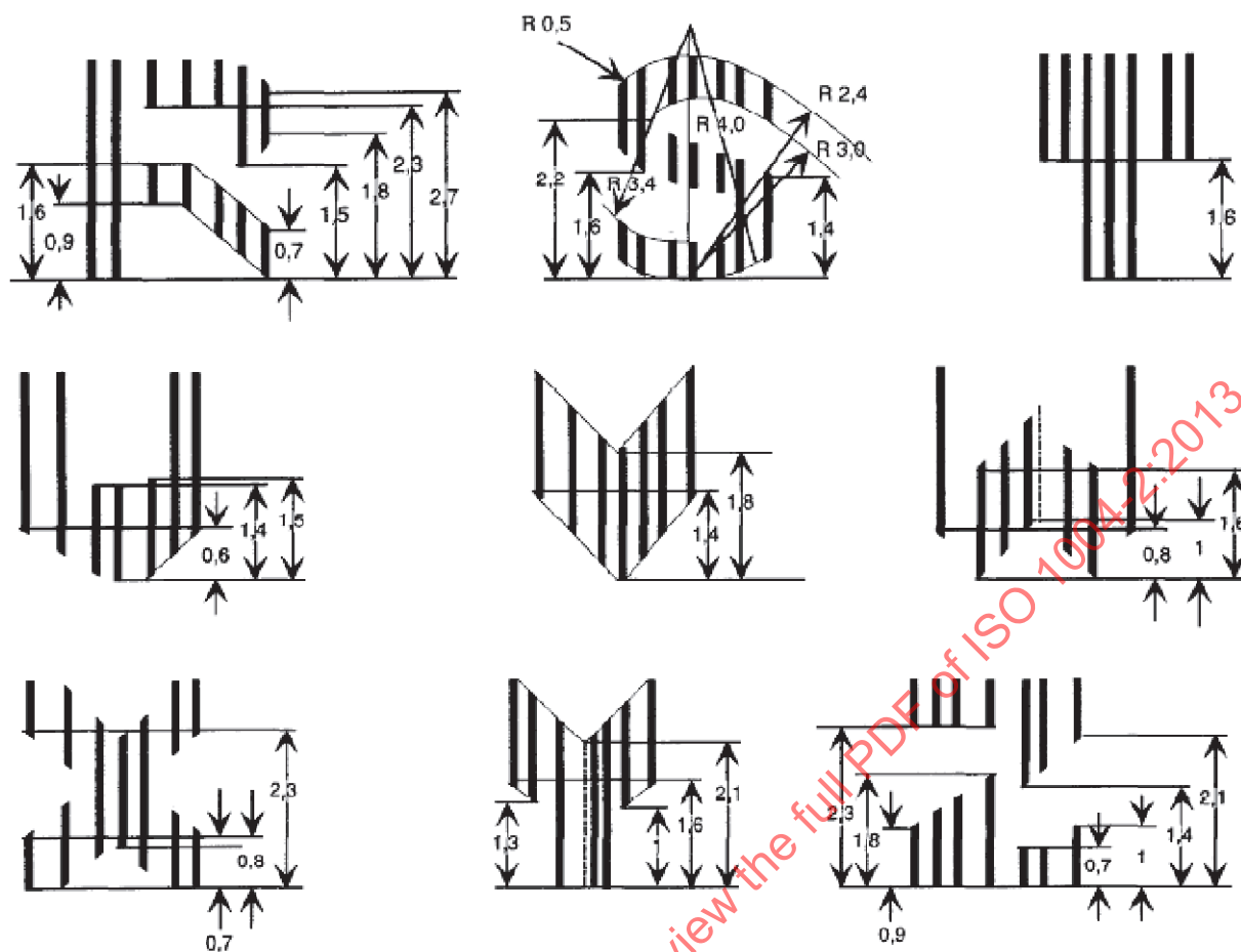
Figure 12 — Letters R to Z: Font height 3,00 mm ( H_{12} )
