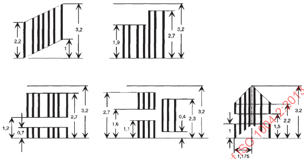
Figure 4 — Symbols: Font height 3,20 mm ( H_{11} ) (top row, left to right: S I, S II; bottom row, left to right: S III, S IV, S V)
