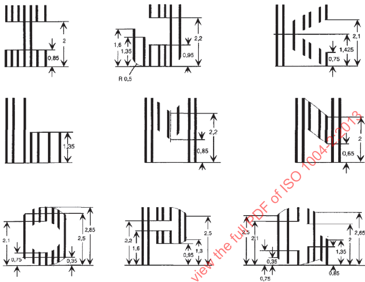
Figure 16 — Letters I to Q: Font height 2,85 mm ( H_{13} )
