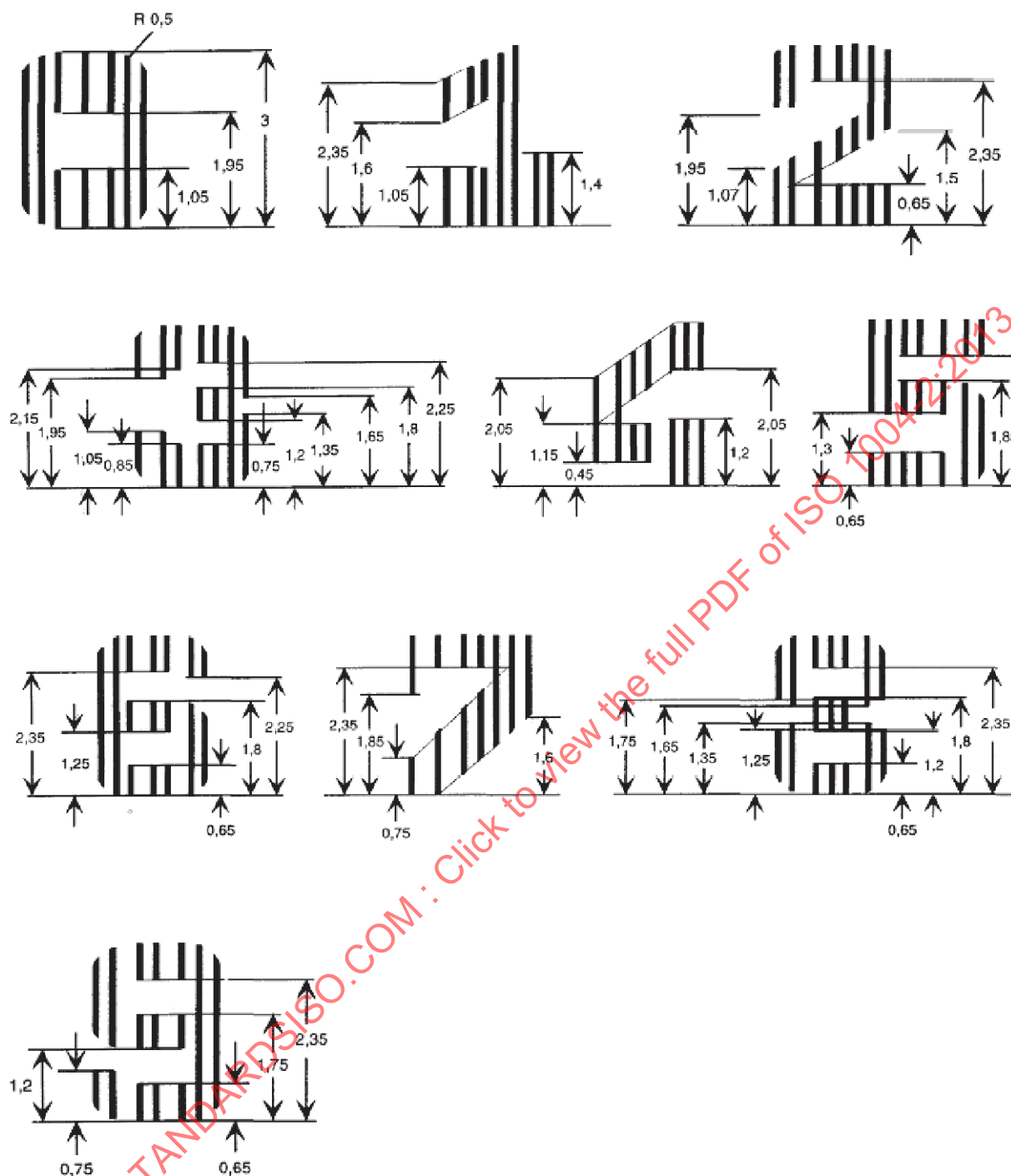
Figure 8 — Digits: Font height 3,00 mm ( H_{12} )
