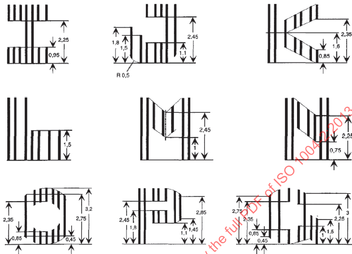
Figure 6 — Letters I to Q: Font height 3,20 mm ( H_{11} )
