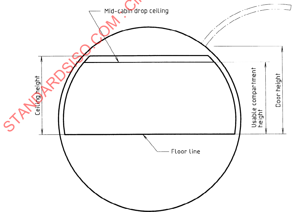
Figure 2 — Main desk compartment usable height
