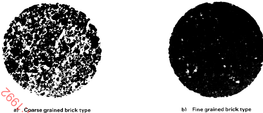
Figure 2 — Carbon or blue paper replica: good
