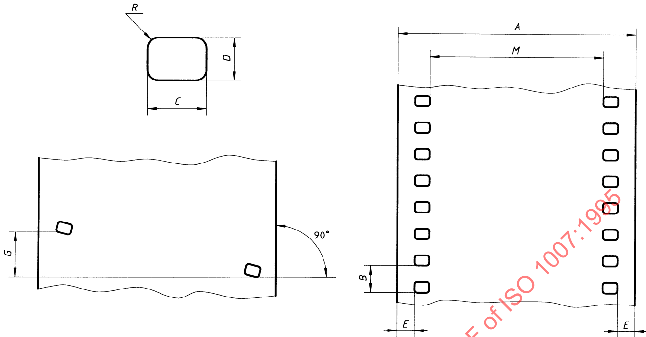
Figure 2 — Perforating dimensions for 135-size film (see table 2)
