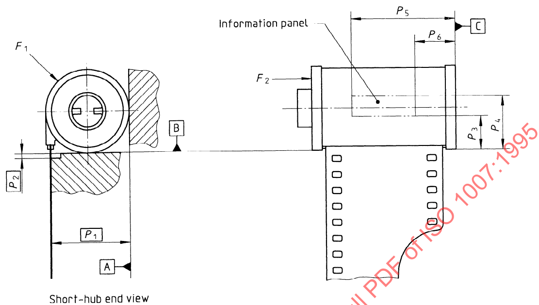
Figure 7 — Dimensions of information panel (see table 14)
